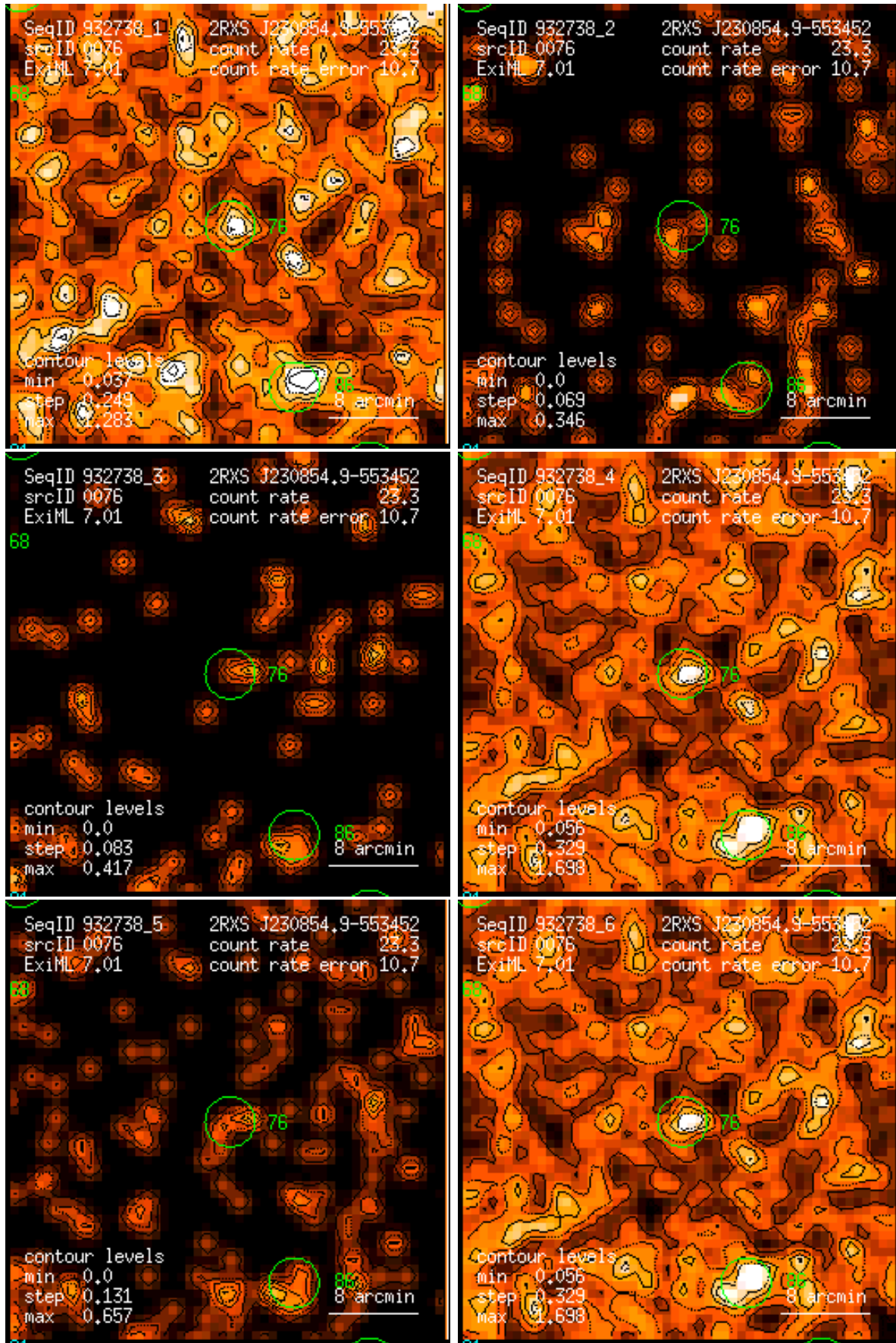
Figure 76: RASS 932738: detection 0076: band rate images, Gaussian filter: (1) PSPC channels 11 – 41, (2) 52 – 90, (3) 91 – 201, (4) 11 – 235, (5) 52 – 201, (6) 11 – 201. Broad band rates in counts/ks. Band rate contour levels in counts/ks/arcmin 2 .
