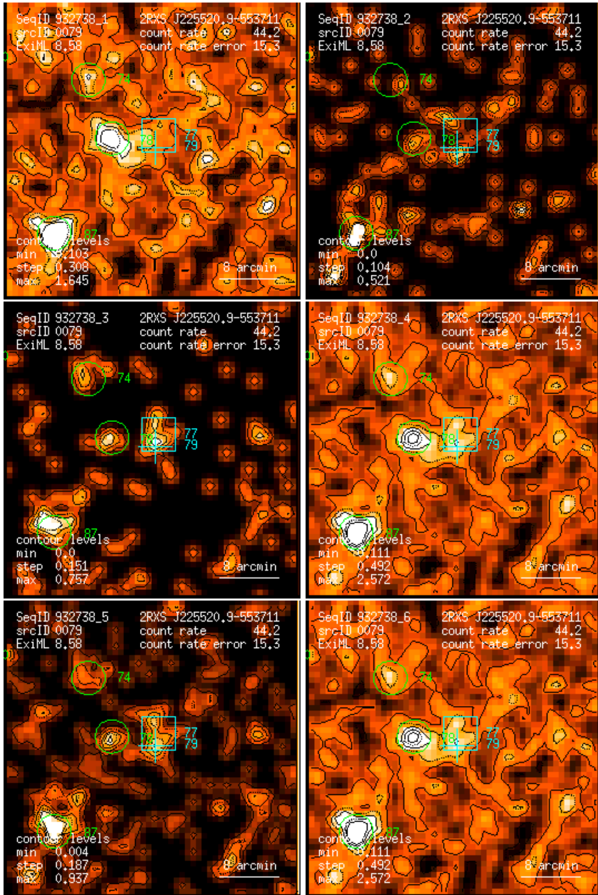
Figure 79: RASS 932738: detection 0079: band rate images, Gaussian filter: (1) PSPC channels 11 – 41, (2) 52 – 90, (3) 91 – 201, (4) 11 – 235, (5) 52 – 201, (6) 11 – 201. Broad band rates in counts/ks. Band rate contour levels in counts/ks/arcmin 2 .
