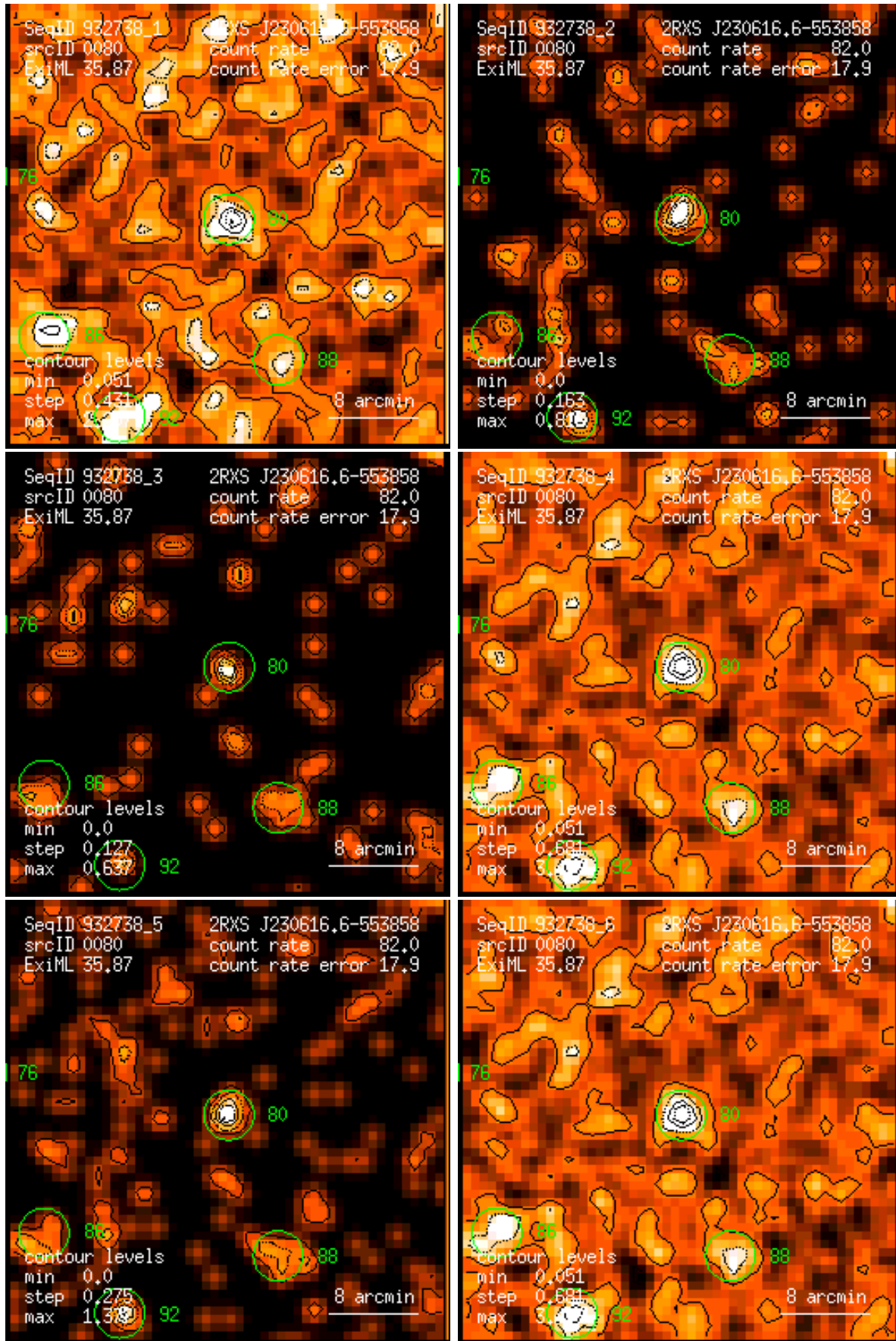
Figure 80: RASS 932738: detection 0080: band rate images, Gaussian filter: (1) PSPC channels 11 – 41, (2) 52 – 90, (3) 91 – 201, (4) 11 – 235, (5) 52 – 201, (6) 11 – 201. Broad band rates in counts/ks. Band rate contour levels in counts/ks/arcmin 2 .
