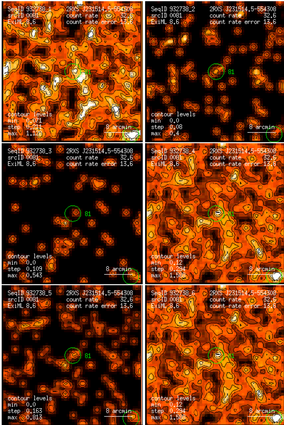
Figure 81: RASS 932738: detection 0081: band rate images, Gaussian filter: (1) PSPC channels 11 – 41, (2) 52 – 90, (3) 91 – 201, (4) 11 – 235, (5) 52 – 201, (6) 11 – 201. Broad band rates in counts/ks. Band rate contour levels in counts/ks/arcmin 2 .
