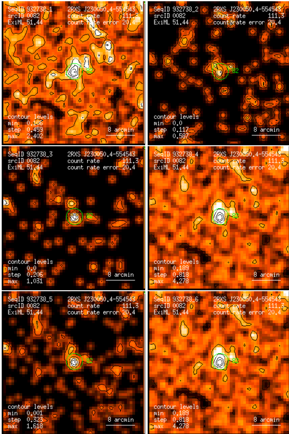
Figure 82: RASS 932738: detection 0082: band rate images, Gaussian filter: (1) PSPC channels 11 – 41, (2) 52 – 90, (3) 91 – 201, (4) 11 – 235, (5) 52 – 201, (6) 11 – 201. Broad band rates in counts/ks. Band rate contour levels in counts/ks/arcmin 2 .
