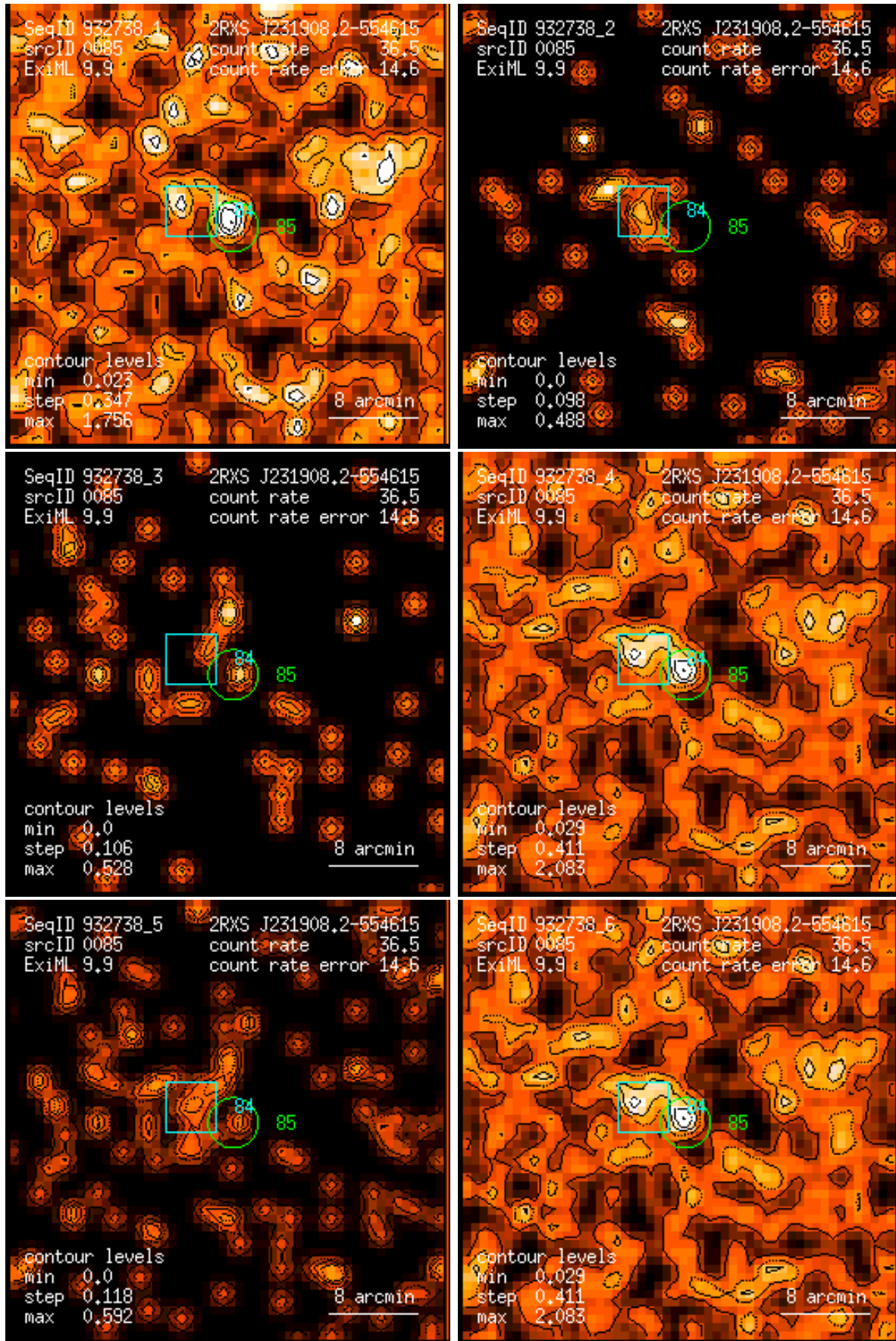
Figure 85: RASS 932738: detection 0085: band rate images, Gaussian filter: (1) PSPC channels 11 – 41, (2) 52 – 90, (3) 91 – 201, (4) 11 – 235, (5) 52 – 201, (6) 11 – 201. Broad band rates in counts/ks. Band rate contour levels in counts/ks/arcmin 2 .
