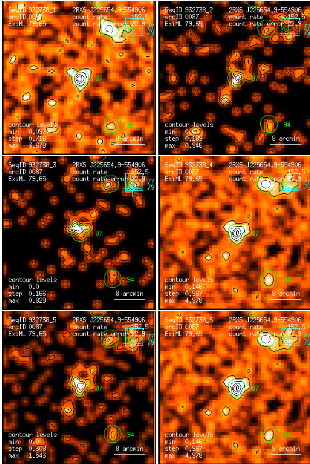
Figure 87: RASS 932738: detection 0087: band rate images, Gaussian filter: (1) PSPC channels 11 – 41, (2) 52 – 90, (3) 91 – 201, (4) 11 – 235, (5) 52 – 201, (6) 11 – 201. Broad band rates in counts/ks. Band rate contour levels in counts/ks/arcmin 2 .
