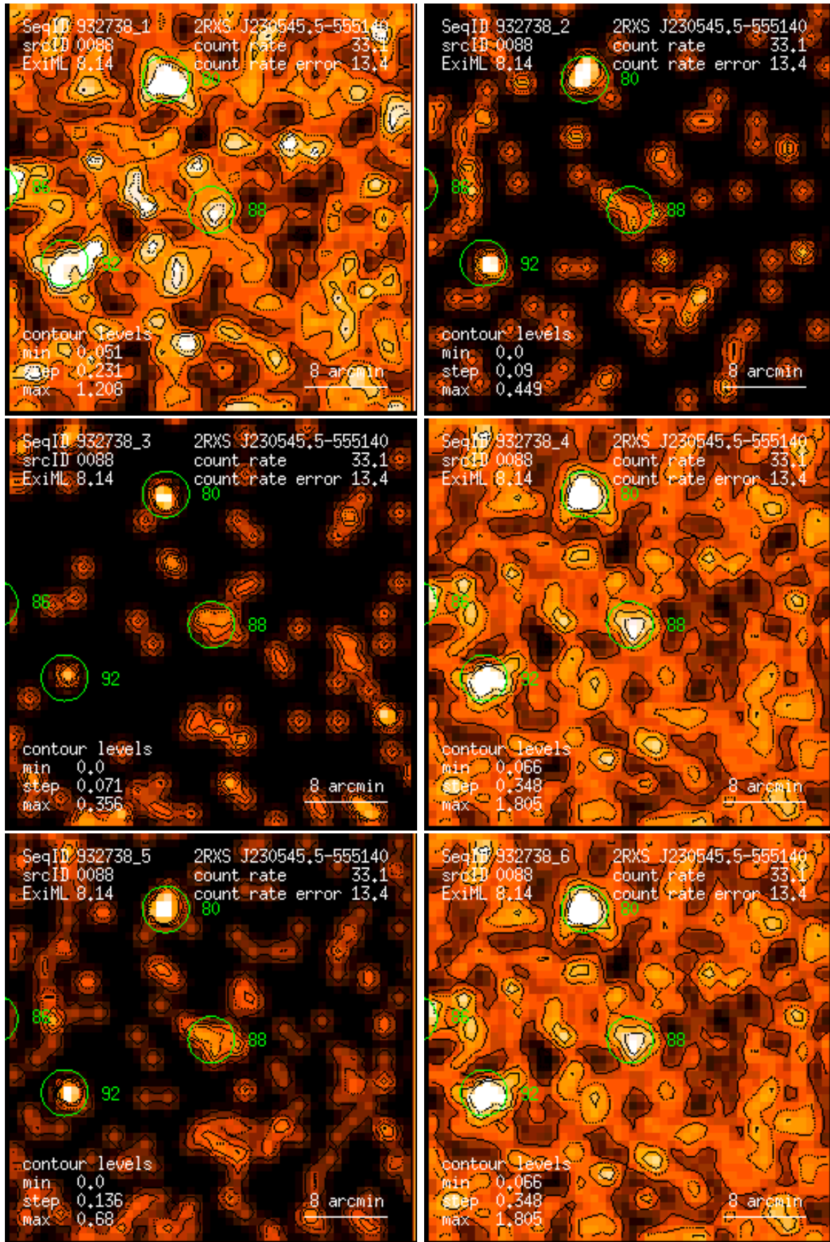
Figure 88: RASS 932738: detection 0088: band rate images, Gaussian filter: (1) PSPC channels 11 – 41, (2) 52 – 90, (3) 91 – 201, (4) 11 – 235, (5) 52 – 201, (6) 11 – 201. Broad band rates in counts/ks. Band rate contour levels in counts/ks/arcmin 2 .
