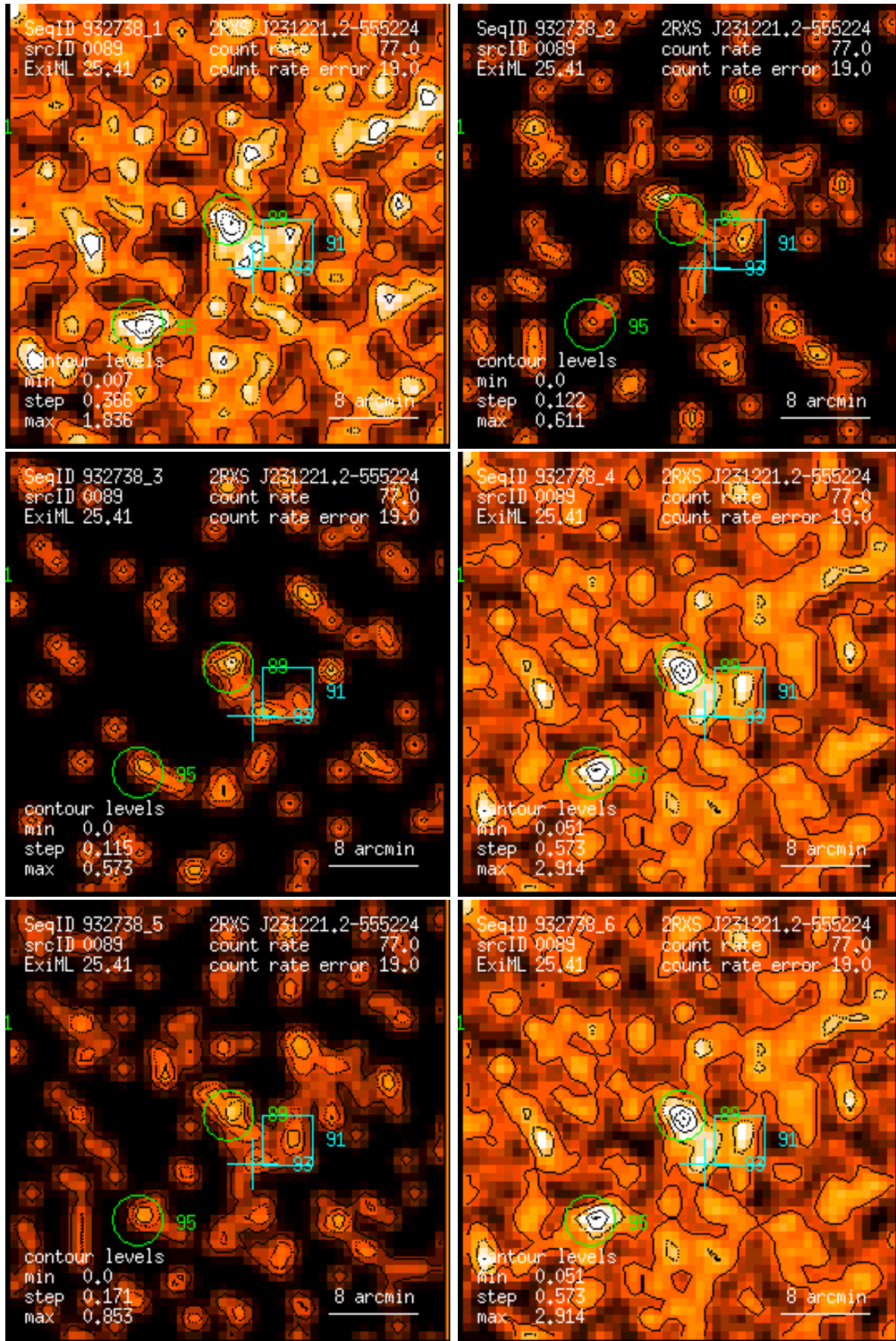
Figure 89: RASS 932738: detection 0089: band rate images, Gaussian filter: (1) PSPC channels 11 – 41, (2) 52 – 90, (3) 91 – 201, (4) 11 – 235, (5) 52 – 201, (6) 11 – 201. Broad band rates in counts/ks. Band rate contour levels in counts/ks/arcmin 2 .
