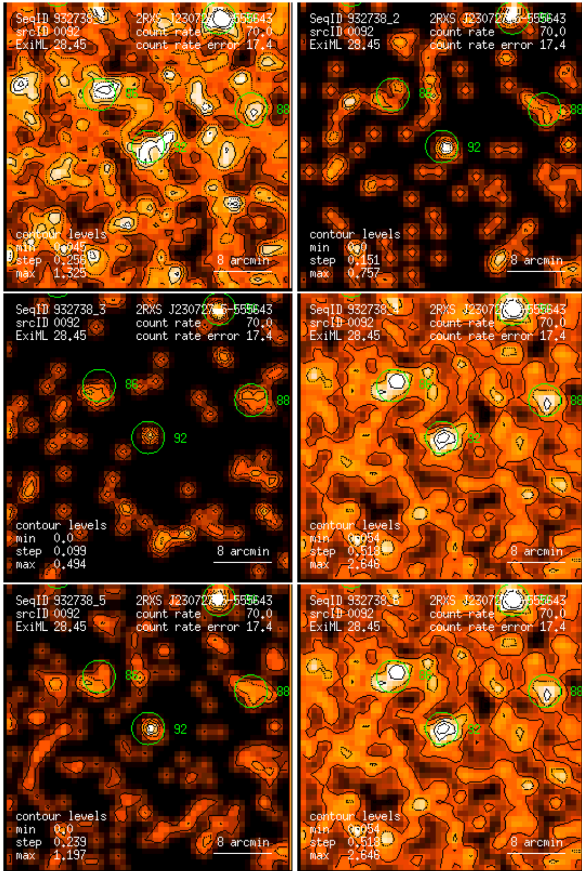
Figure 92: RASS 932738: detection 0092: band rate images, Gaussian filter: (1) PSPC channels 11 – 41, (2) 52 – 90, (3) 91 – 201, (4) 11 – 235, (5) 52 – 201, (6) 11 – 201. Broad band rates in counts/ks. Band rate contour levels in counts/ks/arcmin 2 .
