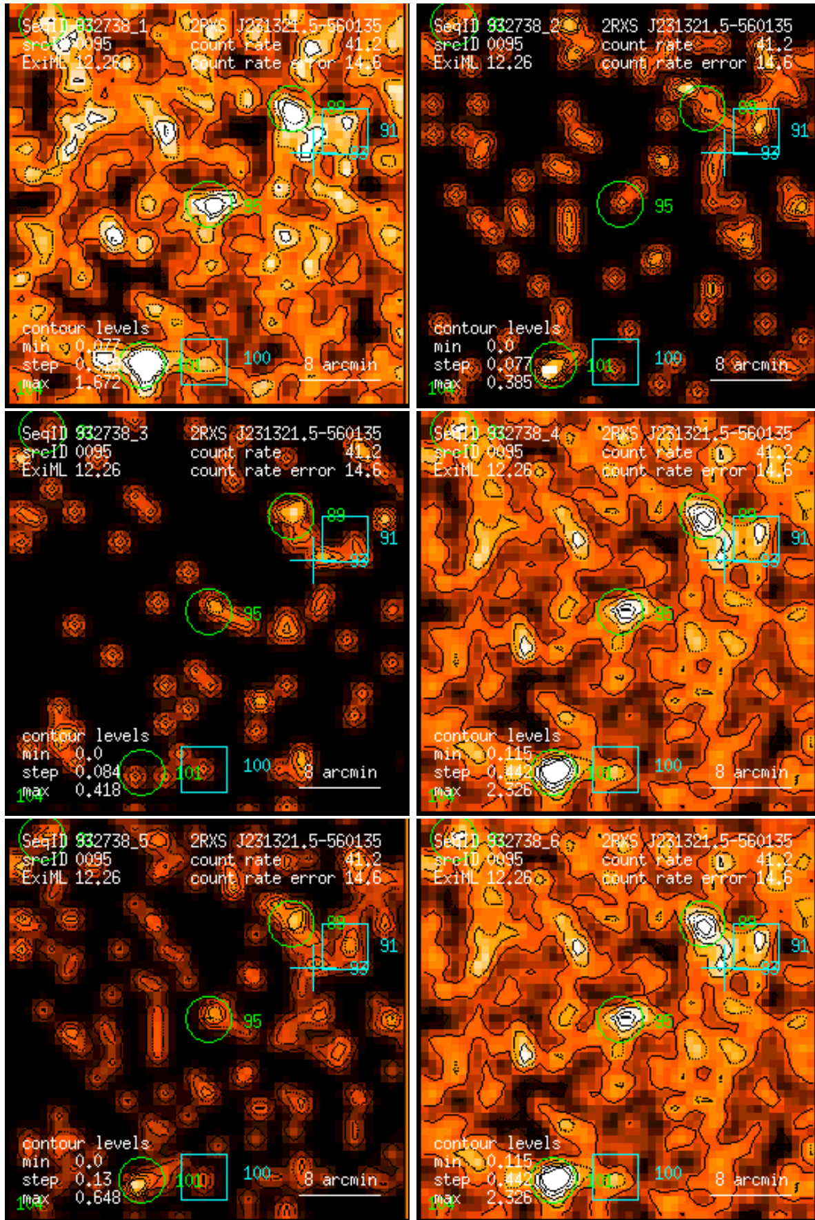
Figure 95: RASS 932738: detection 0095: band rate images, Gaussian filter: (1) PSPC channels 11 – 41, (2) 52 – 90, (3) 91 – 201, (4) 11 – 235, (5) 52 – 201, (6) 11 – 201. Broad band rates in counts/ks. Band rate contour levels in counts/ks/arcmin 2 .
