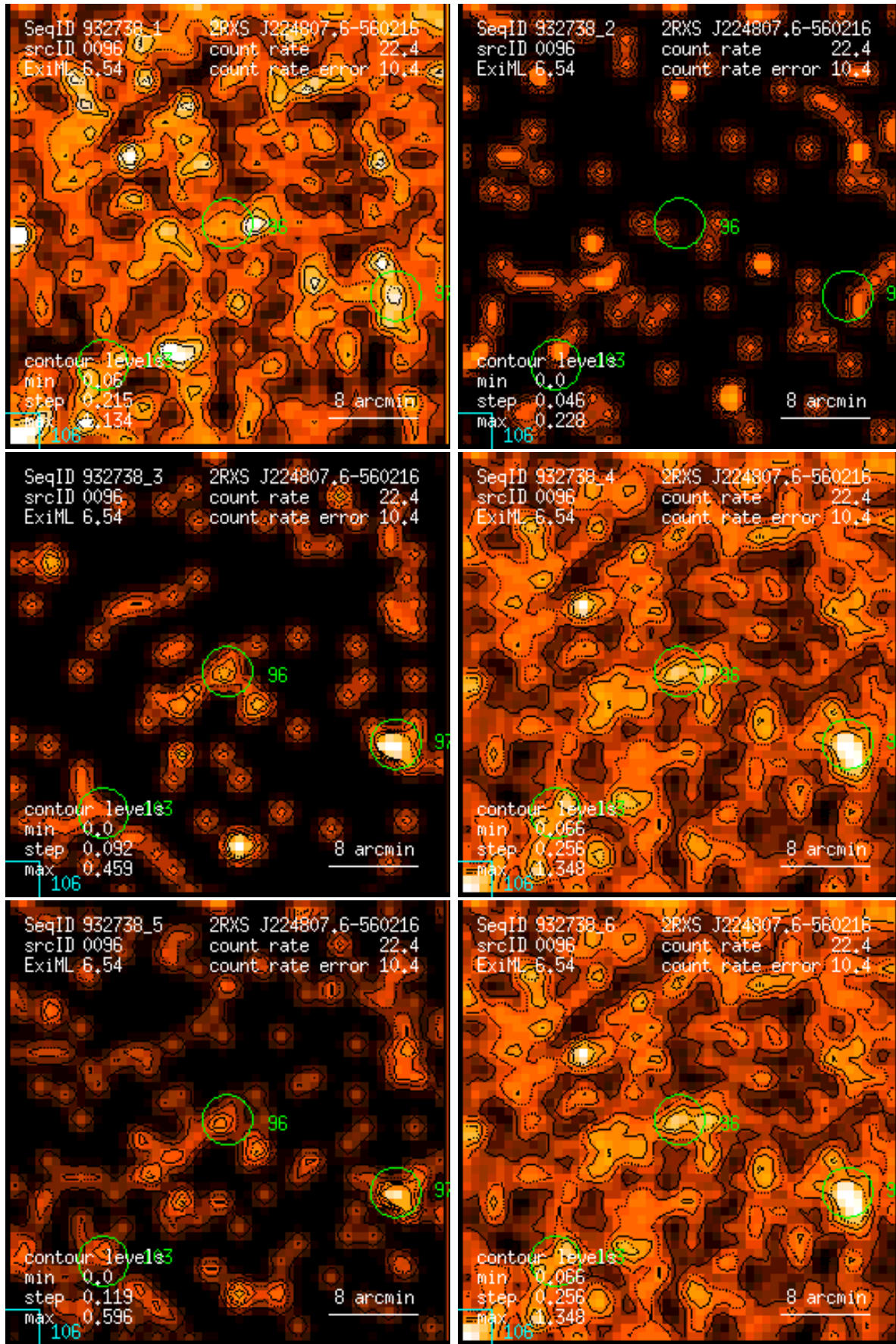
Figure 96: RASS 932738: detection 0096: band rate images, Gaussian filter: (1) PSPC channels 11 – 41, (2) 52 – 90, (3) 91 – 201, (4) 11 – 235, (5) 52 – 201, (6) 11 – 201. Broad band rates in counts/ks. Band rate contour levels in counts/ks/arcmin 2 .
