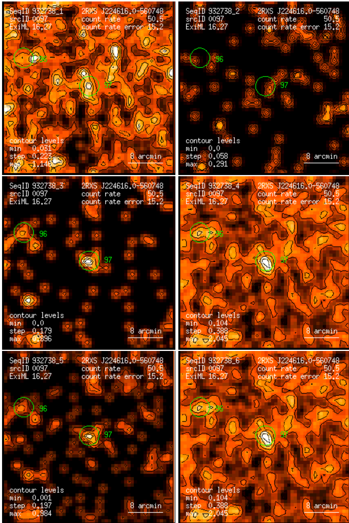
Figure 97: RASS 932738: detection 0097: band rate images, Gaussian filter: (1) PSPC channels 11 – 41, (2) 52 – 90, (3) 91 – 201, (4) 11 – 235, (5) 52 – 201, (6) 11 – 201. Broad band rates in counts/ks. Band rate contour levels in counts/ks/arcmin 2 .
