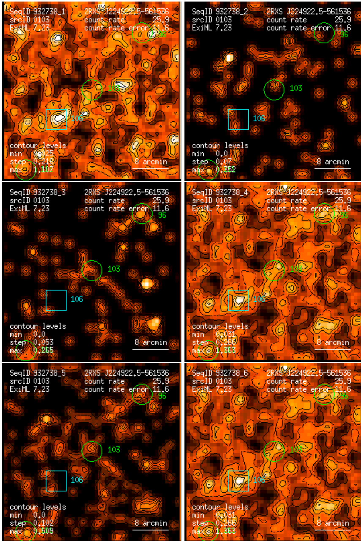
Figure 103: RASS 932738: detection 0103: band rate images, Gaussian filter: (1) PSPC channels 11 – 41, (2) 52 – 90, (3) 91 – 201, (4) 11 – 235, (5) 52 – 201, (6) 11 – 201. Broad band rates in counts/ks. Band rate contour levels in counts/ks/arcmin 2 .
