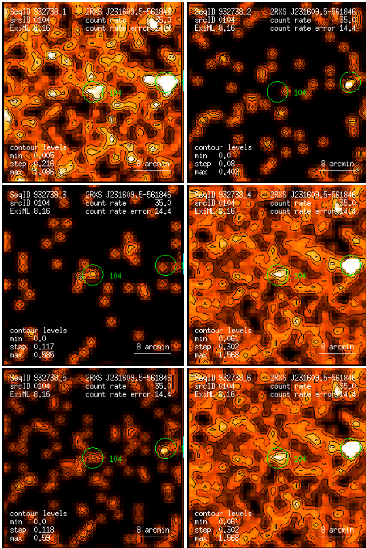
Figure 104: RASS 932738: detection 0104: band rate images, Gaussian filter: (1) PSPC channels 11 – 41, (2) 52 – 90, (3) 91 – 201, (4) 11 – 235, (5) 52 – 201, (6) 11 – 201. Broad band rates in counts/ks. Band rate contour levels in counts/ks/arcmin 2 .
