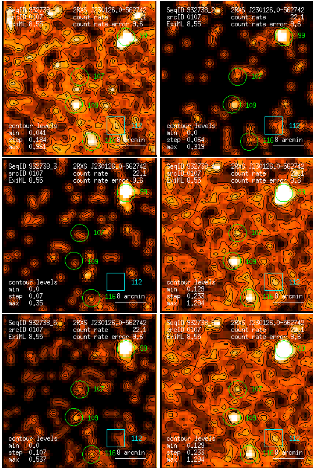
Figure 107: RASS 932738: detection 0107: band rate images, Gaussian filter: (1) PSPC channels 11 – 41, (2) 52 – 90, (3) 91 – 201, (4) 11 – 235, (5) 52 – 201, (6) 11 – 201. Broad band rates in counts/ks. Band rate contour levels in counts/ks/arcmin 2 .
