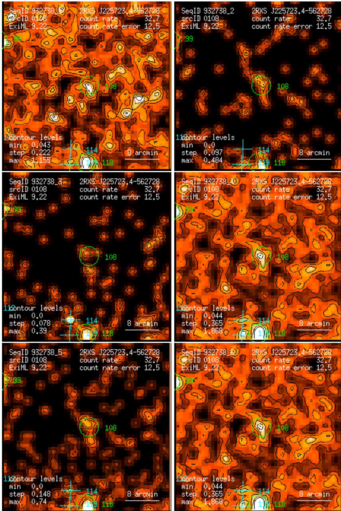
Figure 108: RASS 932738: detection 0108: band rate images, Gaussian filter: (1) PSPC channels 11 – 41, (2) 52 – 90, (3) 91 – 201, (4) 11 – 235, (5) 52 – 201, (6) 11 – 201. Broad band rates in counts/ks. Band rate contour levels in counts/ks/arcmin 2 .
