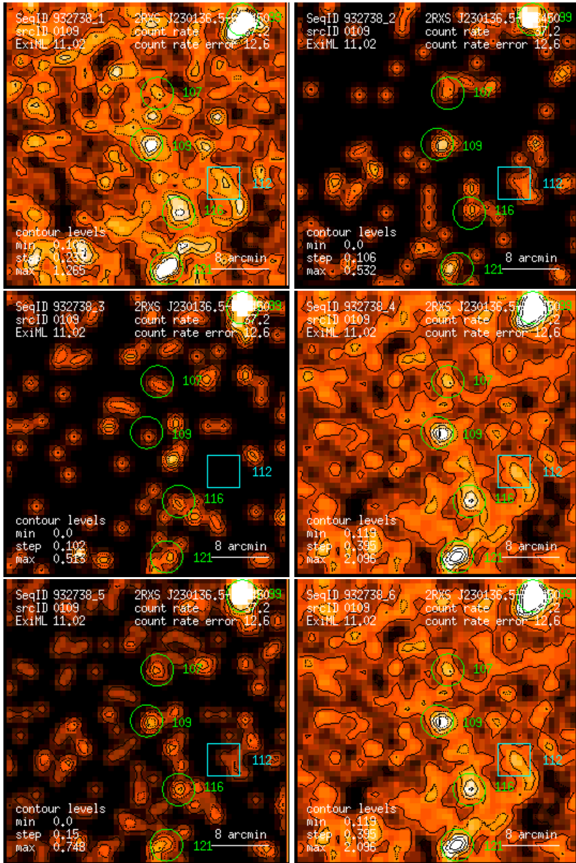
Figure 109: RASS 932738: detection 0109: band rate images, Gaussian filter: (1) PSPC channels 11 – 41, (2) 52 – 90, (3) 91 – 201, (4) 11 – 235, (5) 52 – 201, (6) 11 – 201. Broad band rates in counts/ks. Band rate contour levels in counts/ks/arcmin 2 .
