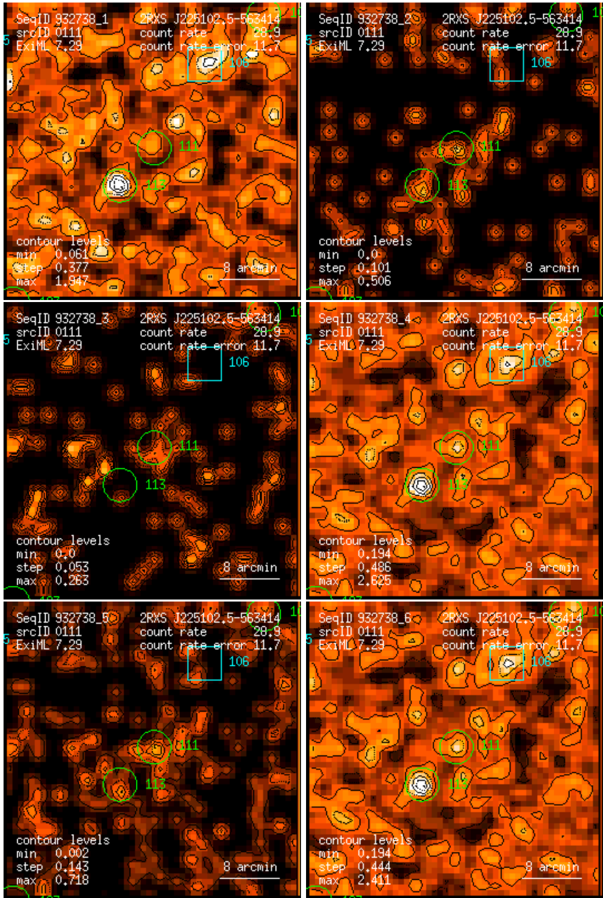
Figure 111: RASS 932738: detection 0111: band rate images, Gaussian filter: (1) PSPC channels 11 – 41, (2) 52 – 90, (3) 91 – 201, (4) 11 – 235, (5) 52 – 201, (6) 11 – 201. Broad band rates in counts/ks. Band rate contour levels in counts/ks/arcmin 2 .
