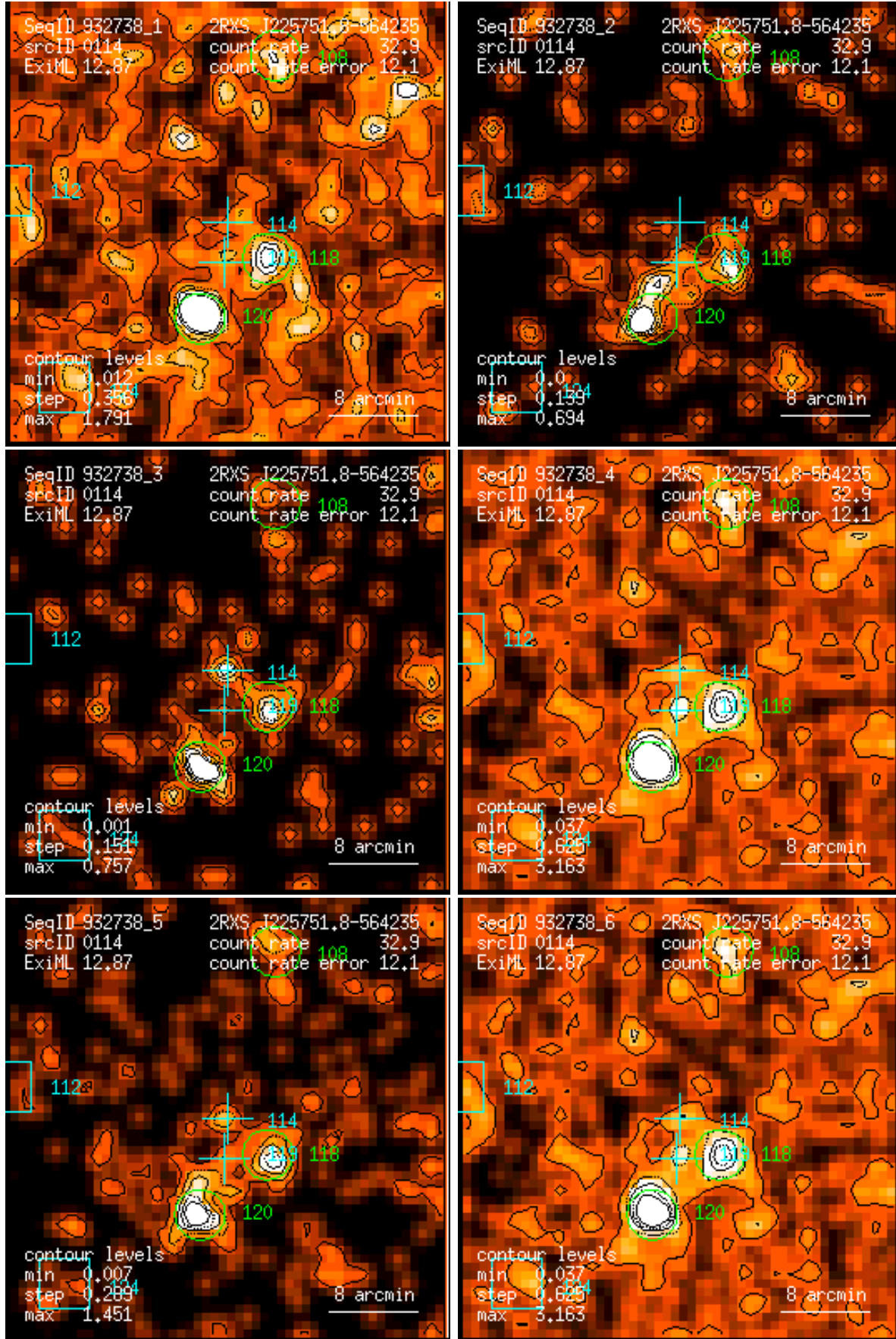
Figure 114: RASS 932738: detection 0114: band rate images, Gaussian filter: (1) PSPC channels 11 – 41, (2) 52 – 90, (3) 91 – 201, (4) 11 – 235, (5) 52 – 201, (6) 11 – 201. Broad band rates in counts/ks. Band rate contour levels in counts/ks/arcmin 2 .
