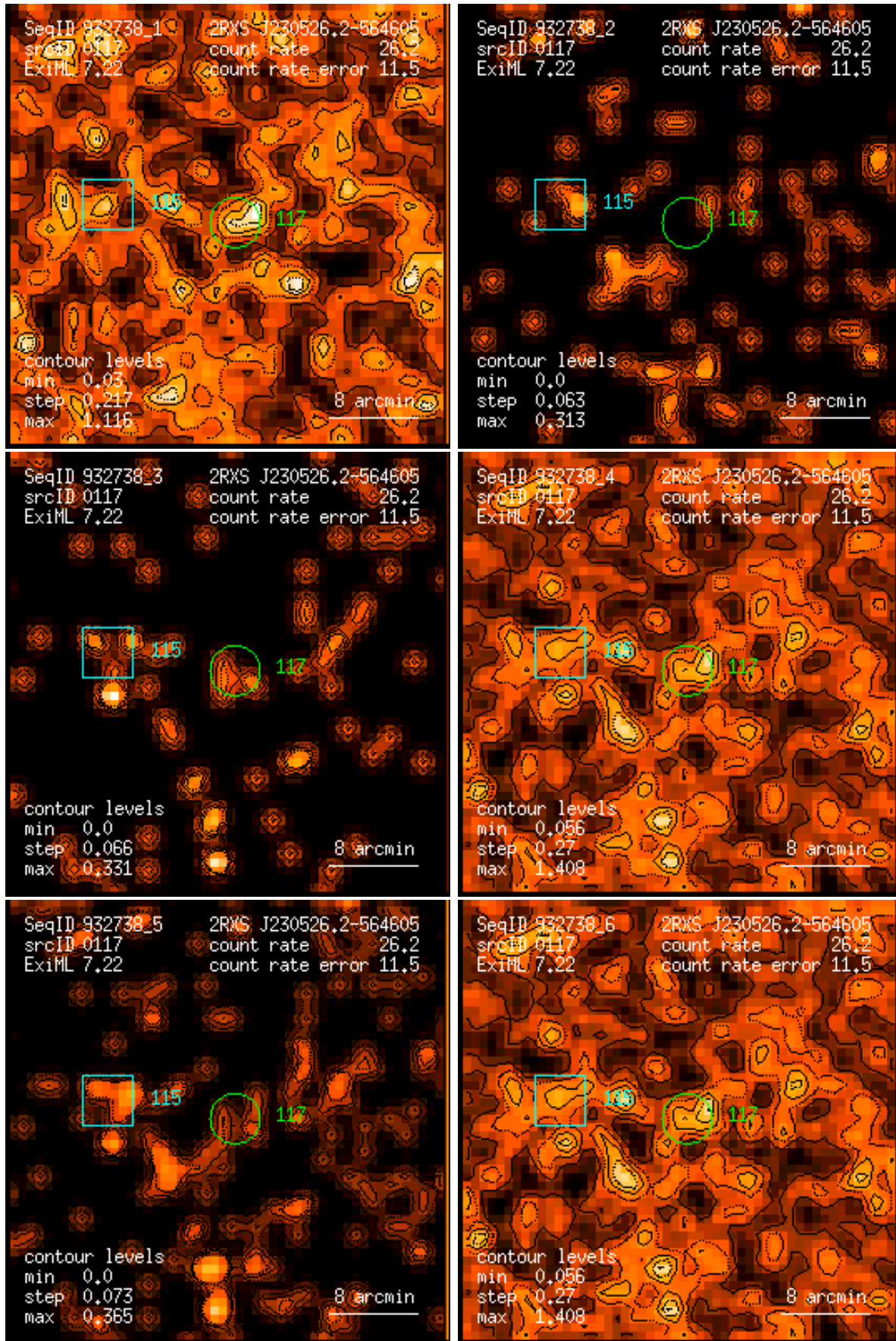
Figure 117: RASS 932738: detection 0117: band rate images, Gaussian filter: (1) PSPC channels 11 – 41, (2) 52 – 90, (3) 91 – 201, (4) 11 – 235, (5) 52 – 201, (6) 11 – 201. Broad band rates in counts/ks. Band rate contour levels in counts/ks/arcmin 2 .
