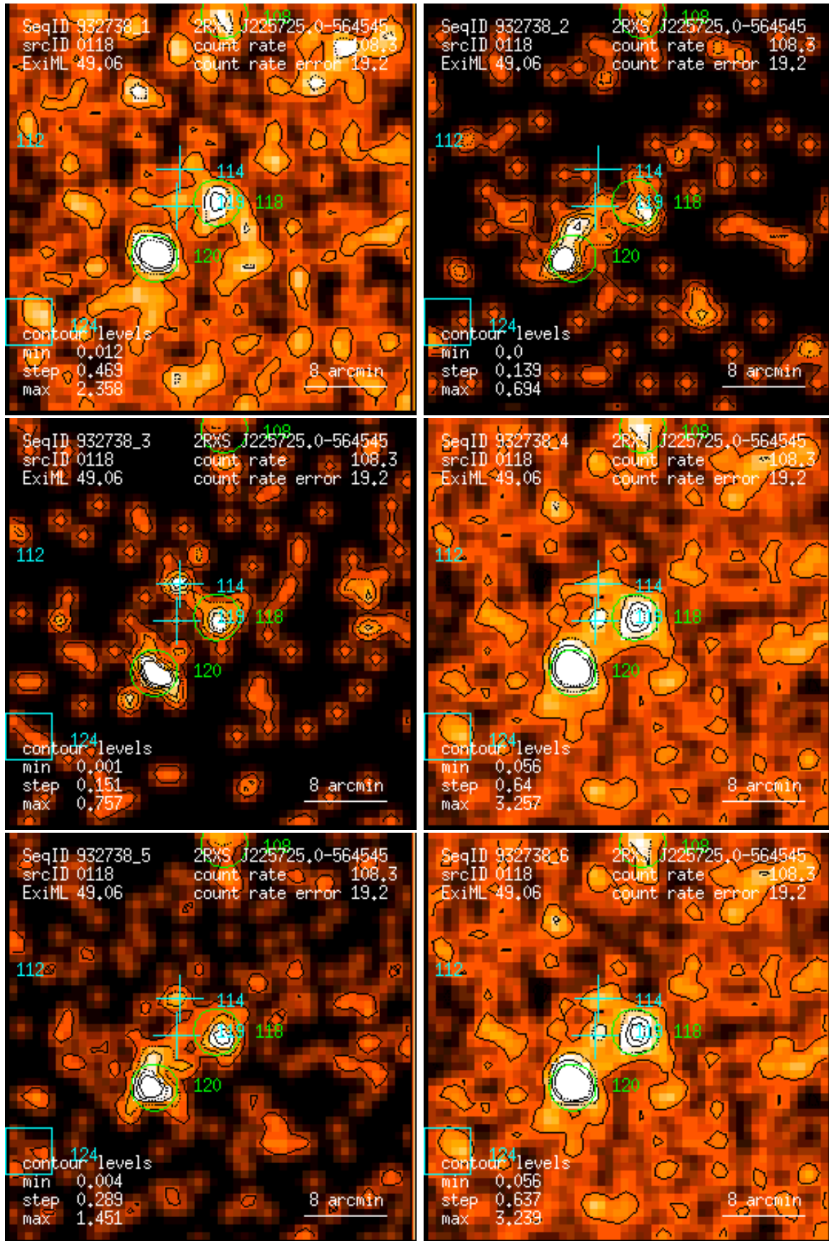
Figure 118: RASS 932738: detection 0118: band rate images, Gaussian filter: (1) PSPC channels 11 – 41, (2) 52 – 90, (3) 91 – 201, (4) 11 – 235, (5) 52 – 201, (6) 11 – 201. Broad band rates in counts/ks. Band rate contour levels in counts/ks/arcmin 2 .
