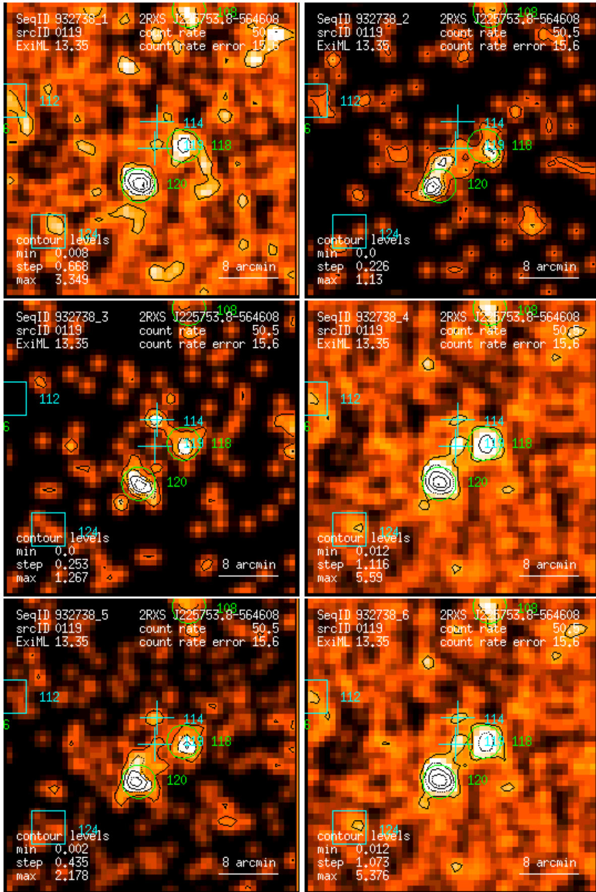
Figure 119: RASS 932738: detection 0119: band rate images, Gaussian filter: (1) PSPC channels 11 – 41, (2) 52 – 90, (3) 91 – 201, (4) 11 – 235, (5) 52 – 201, (6) 11 – 201. Broad band rates in counts/ks. Band rate contour levels in counts/ks/arcmin 2 .
