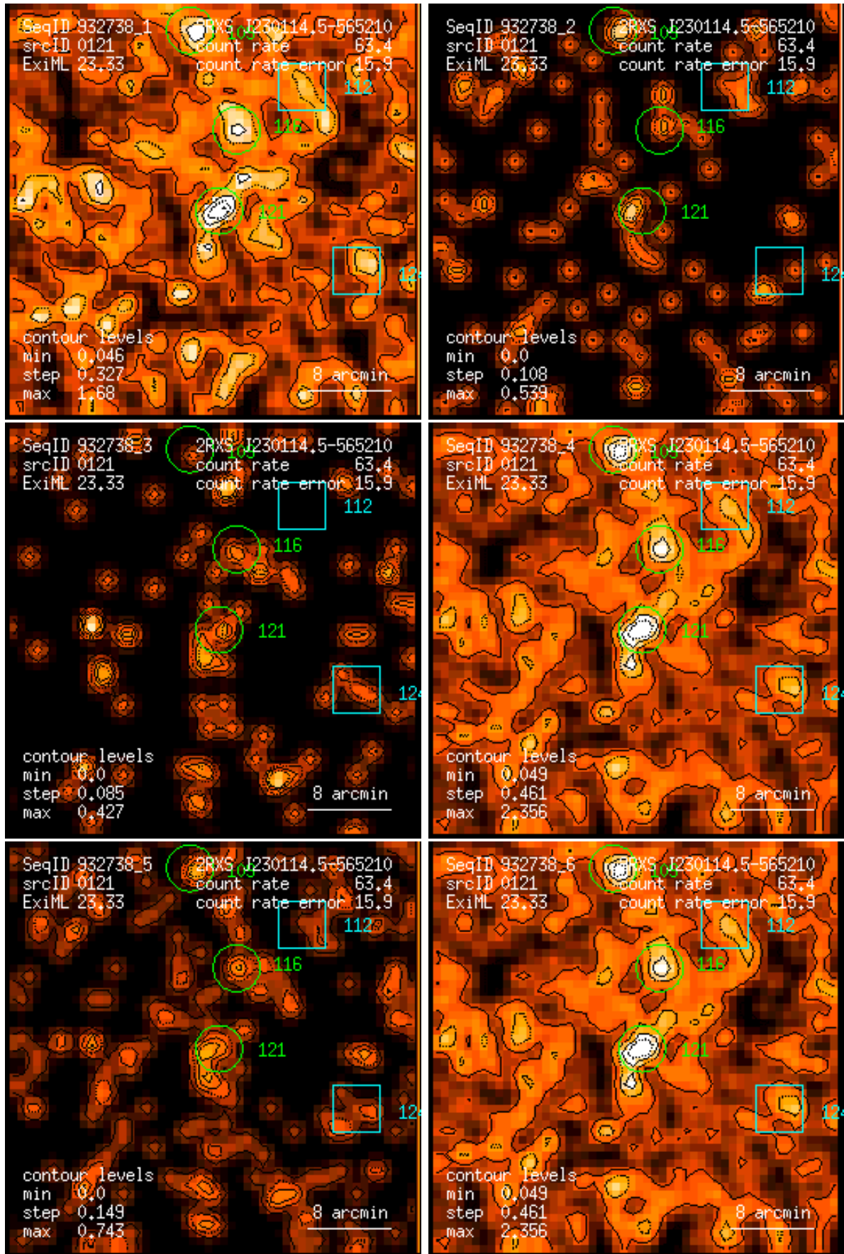
Figure 121: RASS 932738: detection 0121: band rate images, Gaussian filter: (1) PSPC channels 11 – 41, (2) 52 – 90, (3) 91 – 201, (4) 11 – 235, (5) 52 – 201, (6) 11 – 201. Broad band rates in counts/ks. Band rate contour levels in counts/ks/arcmin 2 .
