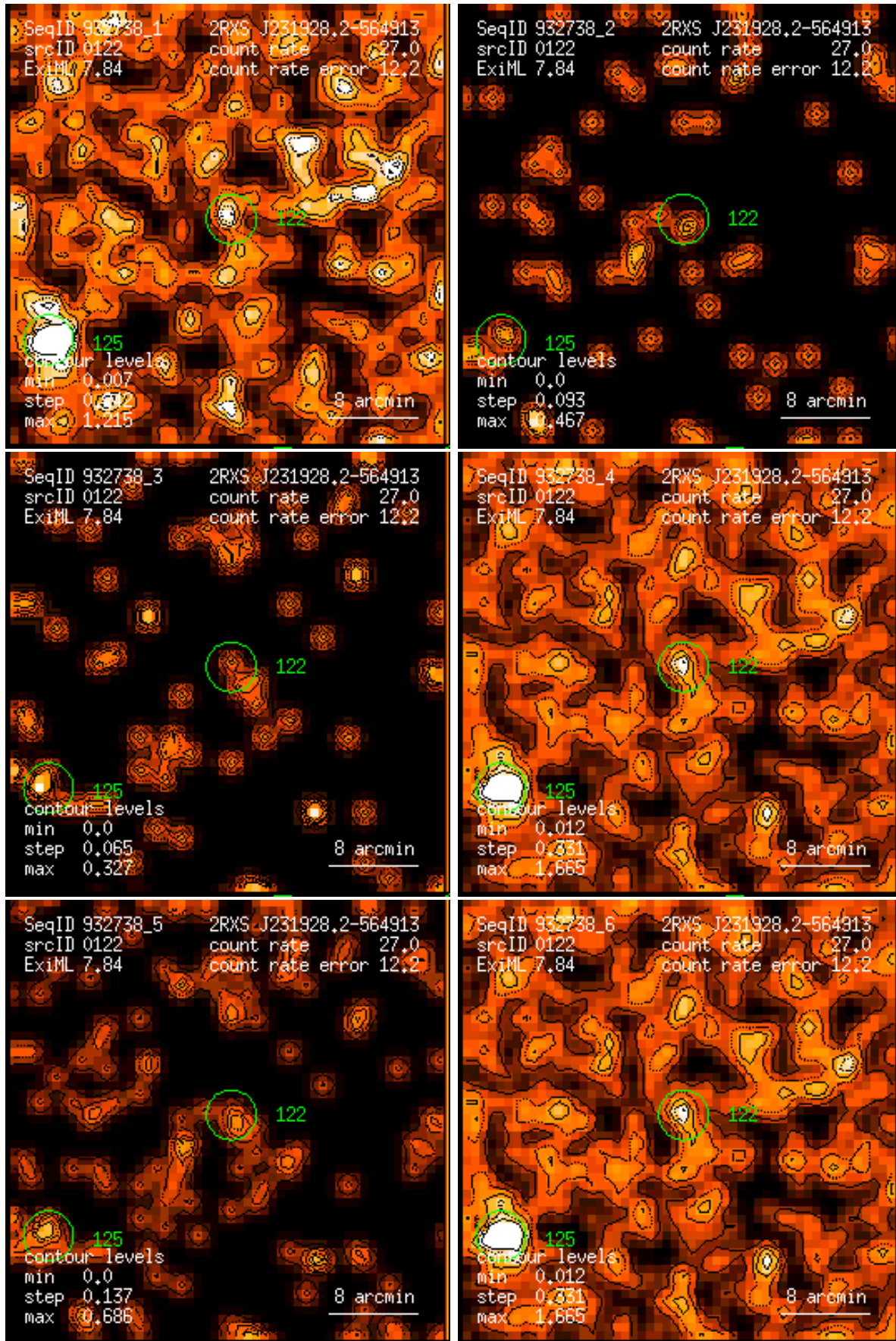
Figure 122: RASS 932738: detection 0122: band rate images, Gaussian filter: (1) PSPC channels 11 – 41, (2) 52 – 90, (3) 91 – 201, (4) 11 – 235, (5) 52 – 201, (6) 11 – 201. Broad band rates in counts/ks. Band rate contour levels in counts/ks/arcmin 2 .
