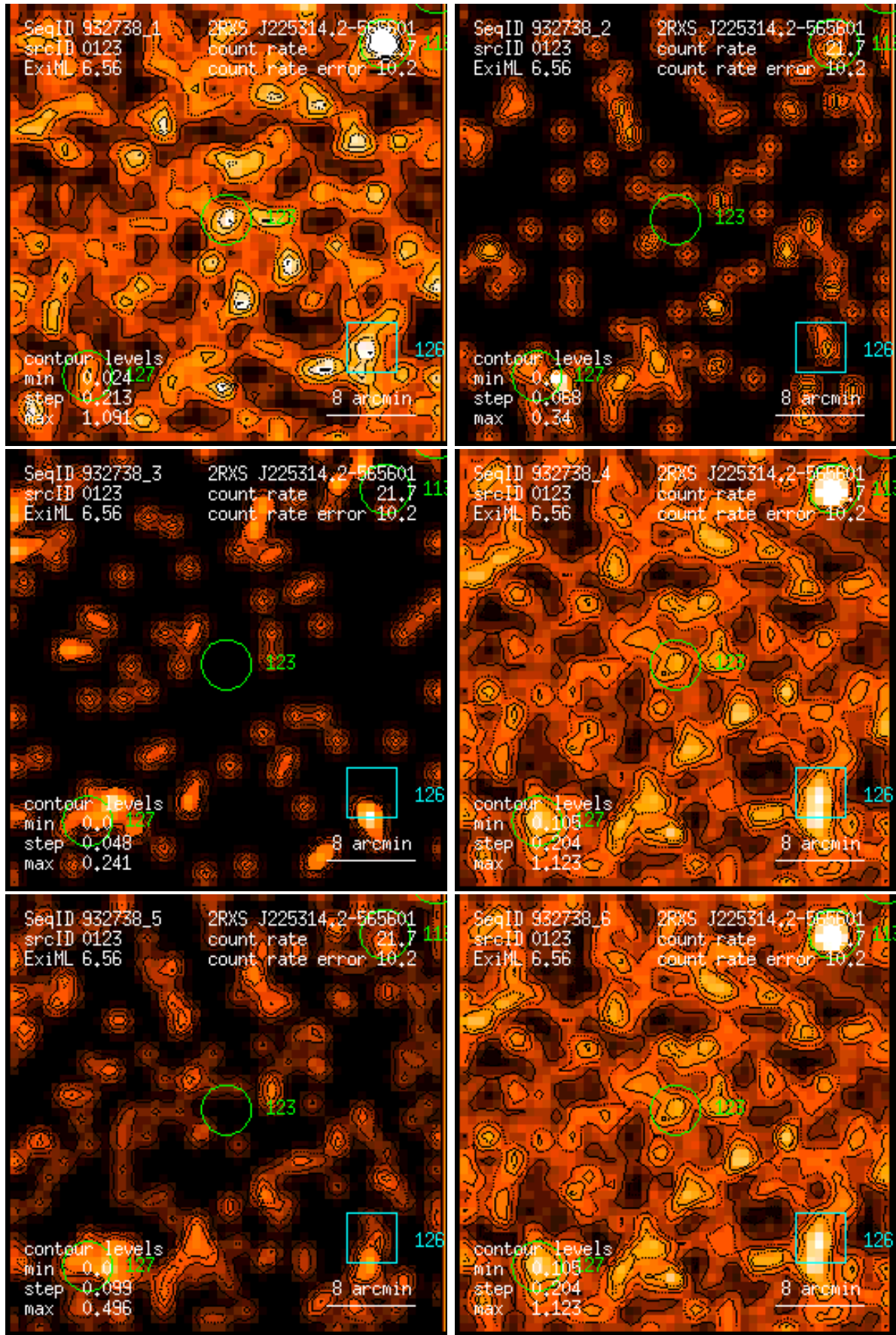
Figure 123: RASS 932738: detection 0123: band rate images, Gaussian filter: (1) PSPC channels 11 – 41, (2) 52 – 90, (3) 91 – 201, (4) 11 – 235, (5) 52 – 201, (6) 11 – 201. Broad band rates in counts/ks. Band rate contour levels in counts/ks/arcmin 2 .
