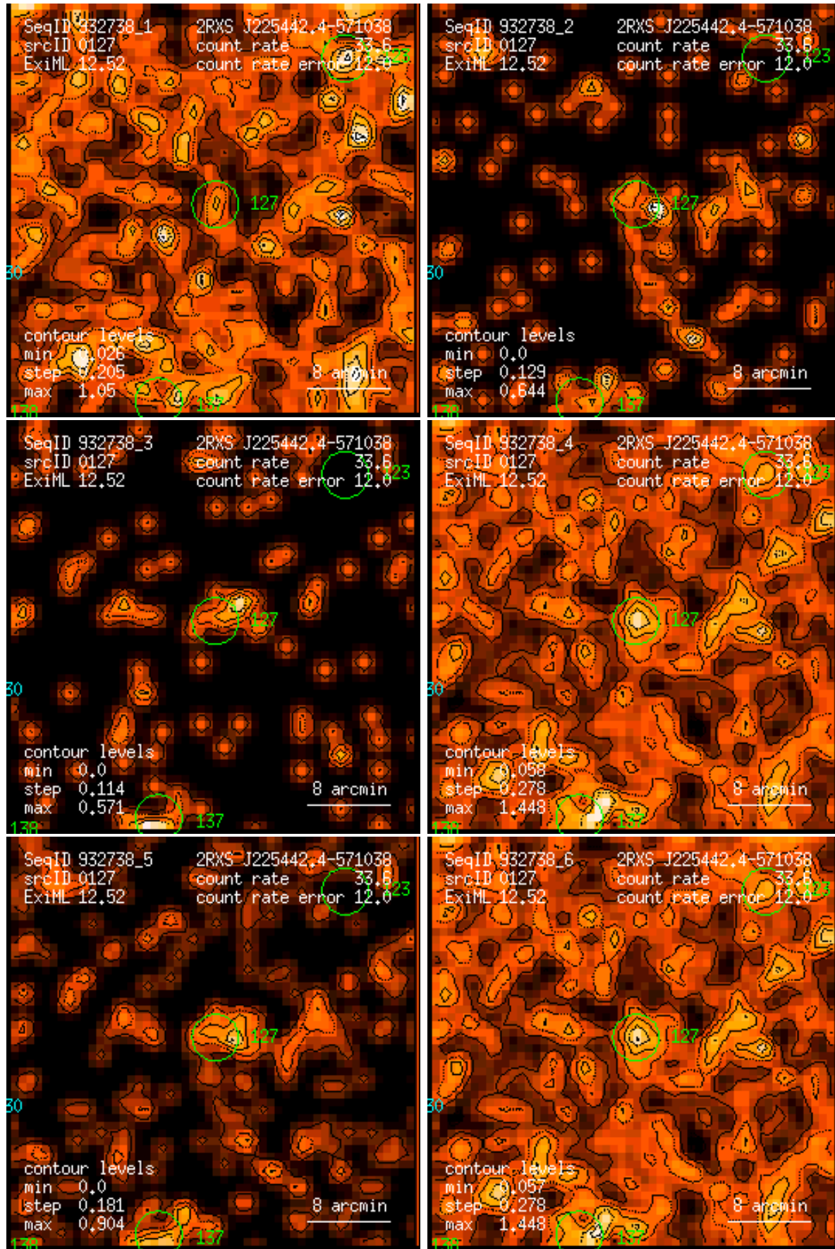
Figure 127: RASS 932738: detection 0127: band rate images, Gaussian filter: (1) PSPC channels 11 – 41, (2) 52 – 90, (3) 91 – 201, (4) 11 – 235, (5) 52 – 201, (6) 11 – 201. Broad band rates in counts/ks. Band rate contour levels in counts/ks/arcmin 2 .
