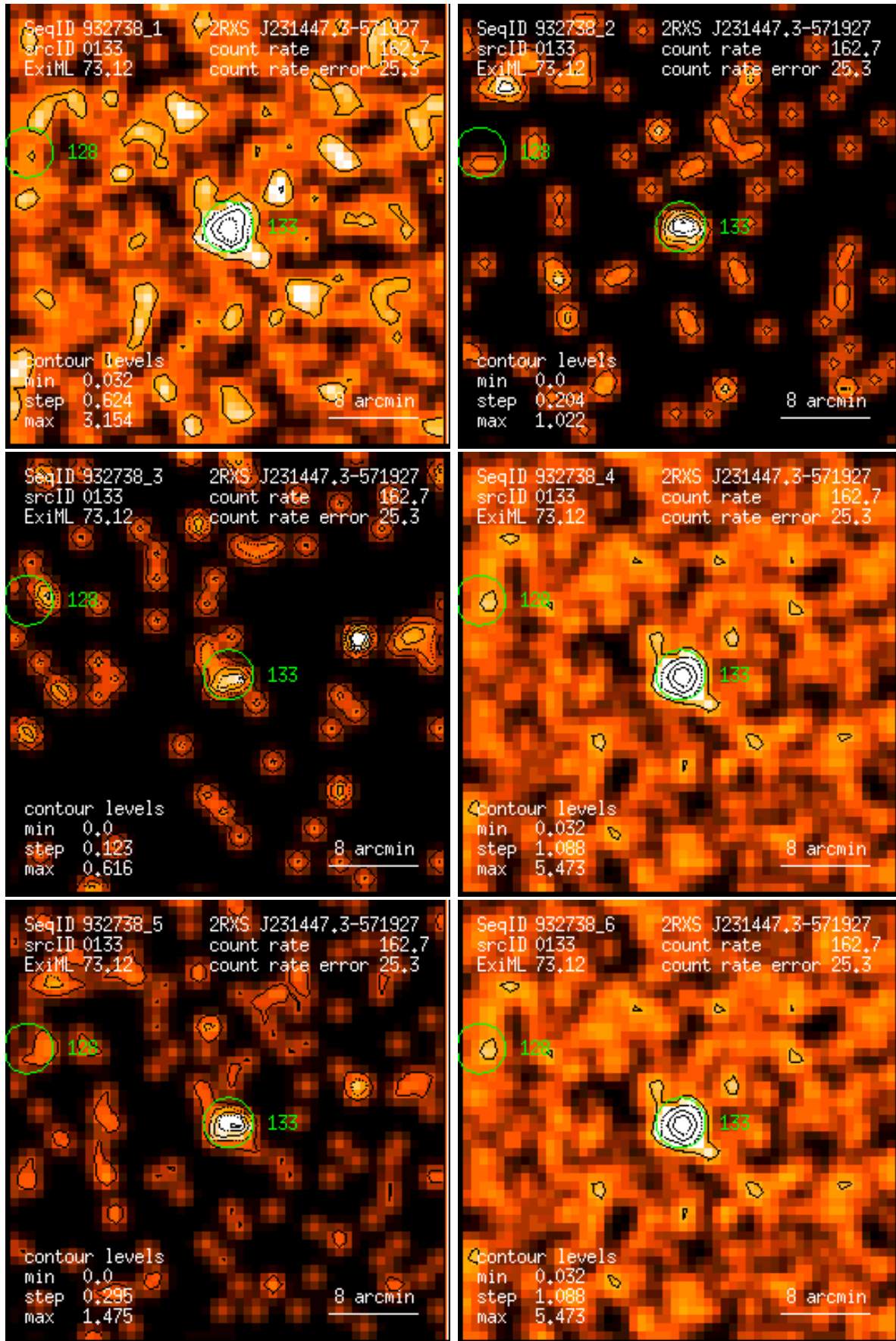
Figure 133: RASS 932738: detection 0133: band rate images, Gaussian filter: (1) PSPC channels 11 – 41, (2) 52 – 90, (3) 91 – 201, (4) 11 – 235, (5) 52 – 201, (6) 11 – 201. Broad band rates in counts/ks. Band rate contour levels in counts/ks/arcmin 2 .
