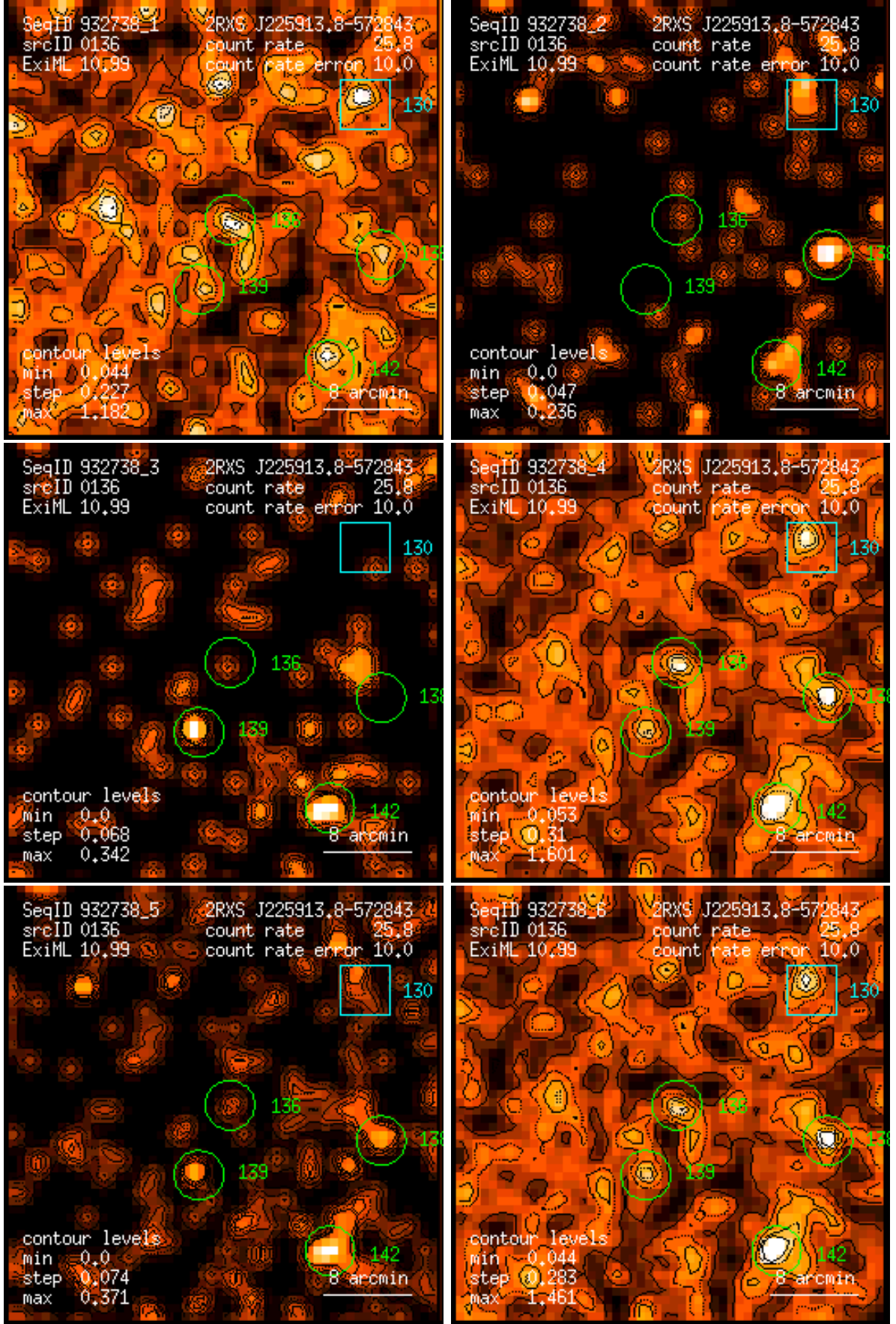
Figure 136: RASS 932738: detection 0136: band rate images, Gaussian filter: (1) PSPC channels 11 – 41, (2) 52 – 90, (3) 91 – 201, (4) 11 – 235, (5) 52 – 201, (6) 11 – 201. Broad band rates in counts/ks. Band rate contour levels in counts/ks/arcmin 2 .
