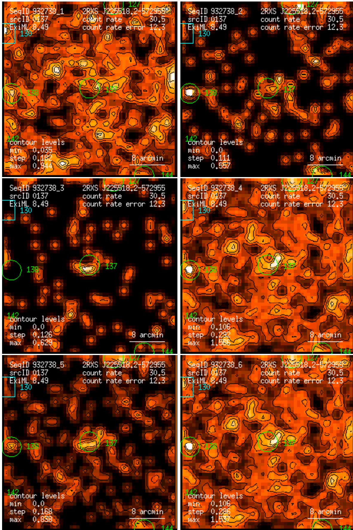
Figure 137: RASS 932738: detection 0137: band rate images, Gaussian filter: (1) PSPC channels 11 – 41, (2) 52 – 90, (3) 91 – 201, (4) 11 – 235, (5) 52 – 201, (6) 11 – 201. Broad band rates in counts/ks. Band rate contour levels in counts/ks/arcmin 2 .
