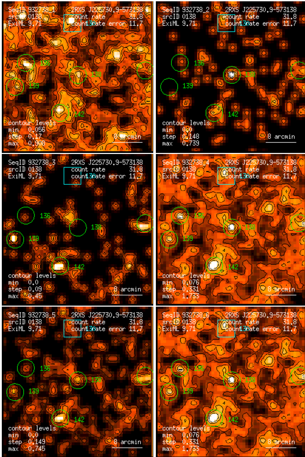
Figure 138: RASS 932738: detection 0138: band rate images, Gaussian filter: (1) PSPC channels 11 – 41, (2) 52 – 90, (3) 91 – 201, (4) 11 – 235, (5) 52 – 201, (6) 11 – 201. Broad band rates in counts/ks. Band rate contour levels in counts/ks/arcmin 2 .
