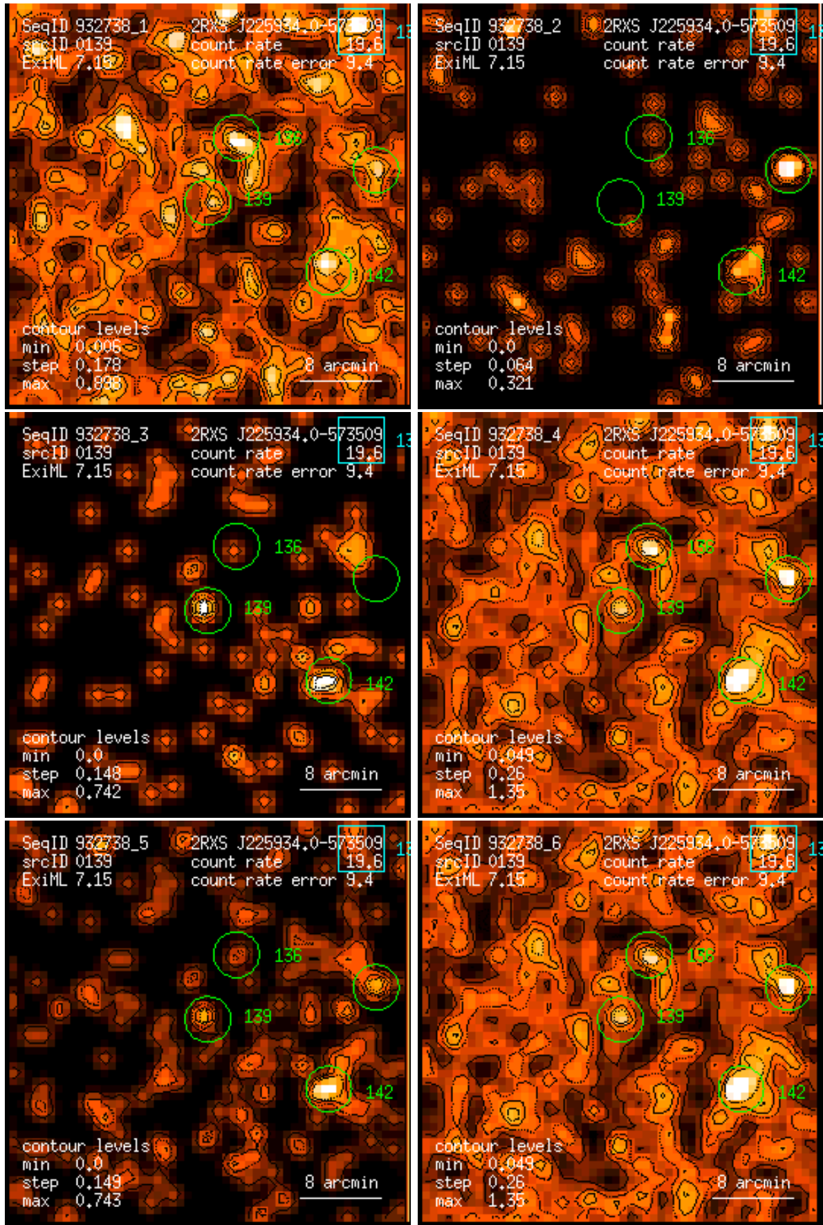
Figure 139: RASS 932738: detection 0139: band rate images, Gaussian filter: (1) PSPC channels 11 – 41, (2) 52 – 90, (3) 91 – 201, (4) 11 – 235, (5) 52 – 201, (6) 11 – 201. Broad band rates in counts/ks. Band rate contour levels in counts/ks/arcmin 2 .
