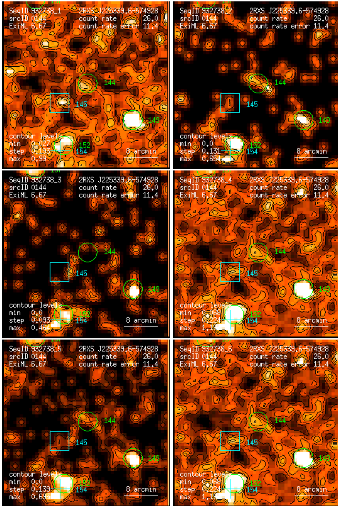
Figure 144: RASS 932738: detection 0144: band rate images, Gaussian filter: (1) PSPC channels 11 – 41, (2) 52 – 90, (3) 91 – 201, (4) 11 – 235, (5) 52 – 201, (6) 11 – 201. Broad band rates in counts/ks. Band rate contour levels in counts/ks/arcmin 2 .
