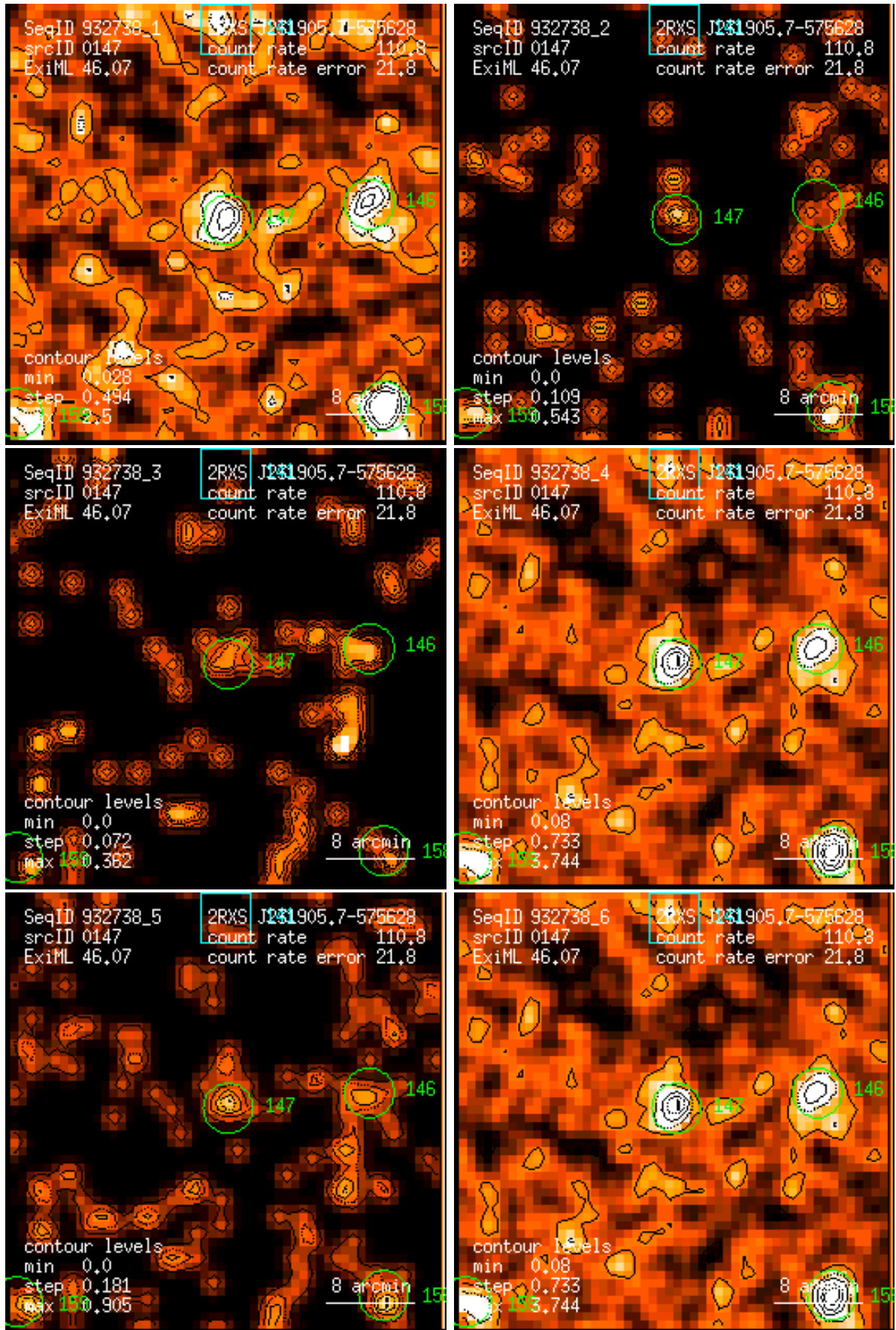
Figure 147: RASS 932738: detection 0147: band rate images, Gaussian filter: (1) PSPC channels 11 – 41, (2) 52 – 90, (3) 91 – 201, (4) 11 – 235, (5) 52 – 201, (6) 11 – 201. Broad band rates in counts/ks. Band rate contour levels in counts/ks/arcmin 2 .
