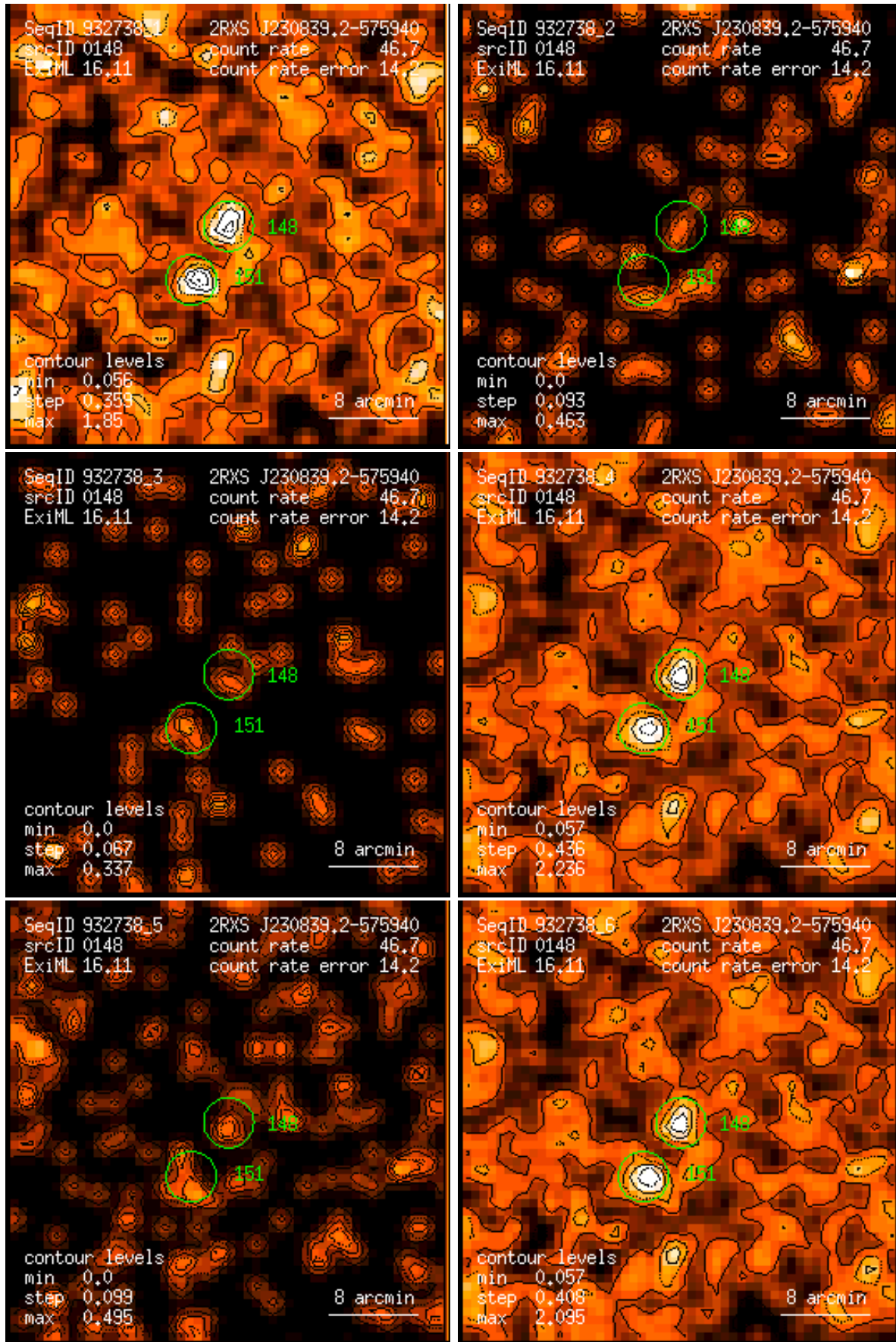
Figure 148: RASS 932738: detection 0148: band rate images, Gaussian filter: (1) PSPC channels 11 – 41, (2) 52 – 90, (3) 91 – 201, (4) 11 – 235, (5) 52 – 201, (6) 11 – 201. Broad band rates in counts/ks. Band rate contour levels in counts/ks/arcmin 2 .
