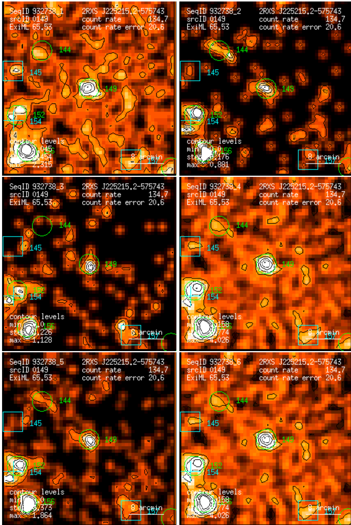
Figure 149: RASS 932738: detection 0149: band rate images, Gaussian filter: (1) PSPC channels 11 – 41, (2) 52 – 90, (3) 91 – 201, (4) 11 – 235, (5) 52 – 201, (6) 11 – 201. Broad band rates in counts/ks. Band rate contour levels in counts/ks/arcmin 2 .
