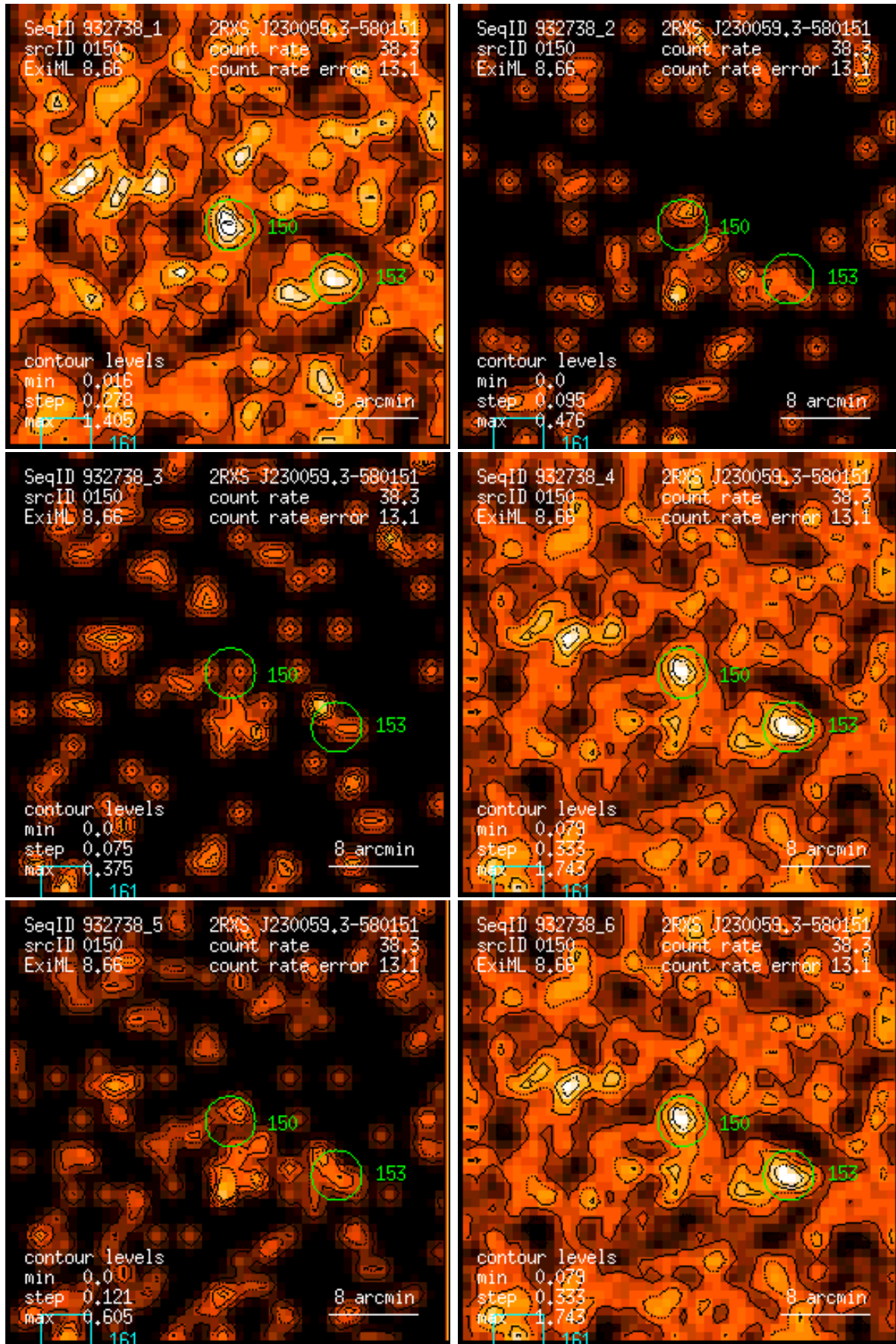
Figure 150: RASS 932738: detection 0150: band rate images, Gaussian filter: (1) PSPC channels 11 – 41, (2) 52 – 90, (3) 91 – 201, (4) 11 – 235, (5) 52 – 201, (6) 11 – 201. Broad band rates in counts/ks. Band rate contour levels in counts/ks/arcmin 2 .
