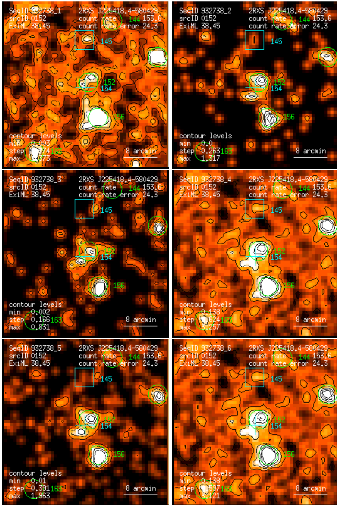
Figure 152: RASS 932738: detection 0152: band rate images, Gaussian filter: (1) PSPC channels 11 – 41, (2) 52 – 90, (3) 91 – 201, (4) 11 – 235, (5) 52 – 201, (6) 11 – 201. Broad band rates in counts/ks. Band rate contour levels in counts/ks/arcmin 2 .
