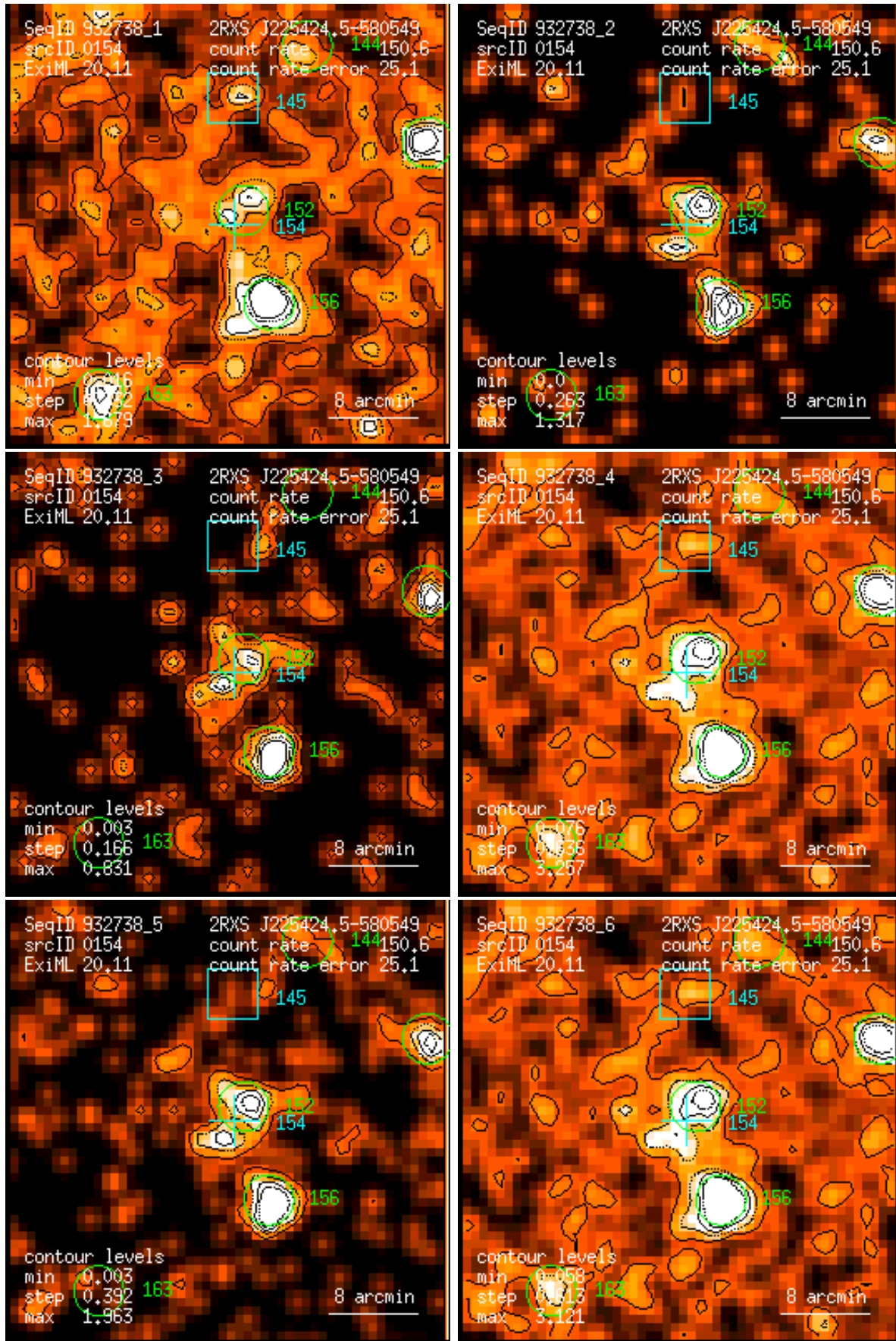
Figure 154: RASS 932738: detection 0154: band rate images, Gaussian filter: (1) PSPC channels 11 – 41, (2) 52 – 90, (3) 91 – 201, (4) 11 – 235, (5) 52 – 201, (6) 11 – 201. Broad band rates in counts/ks. Band rate contour levels in counts/ks/arcmin 2 .
