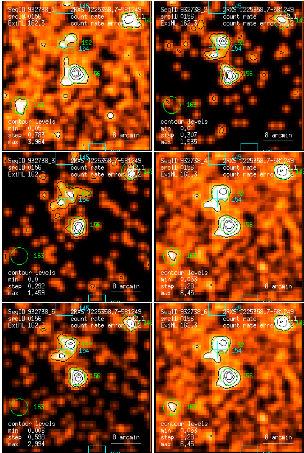
Figure 156: RASS 932738: detection 0156: band rate images, Gaussian filter: (1) PSPC channels 11 – 41, (2) 52 – 90, (3) 91 – 201, (4) 11 – 235, (5) 52 – 201, (6) 11 – 201. Broad band rates in counts/ks. Band rate contour levels in counts/ks/arcmin 2 .
