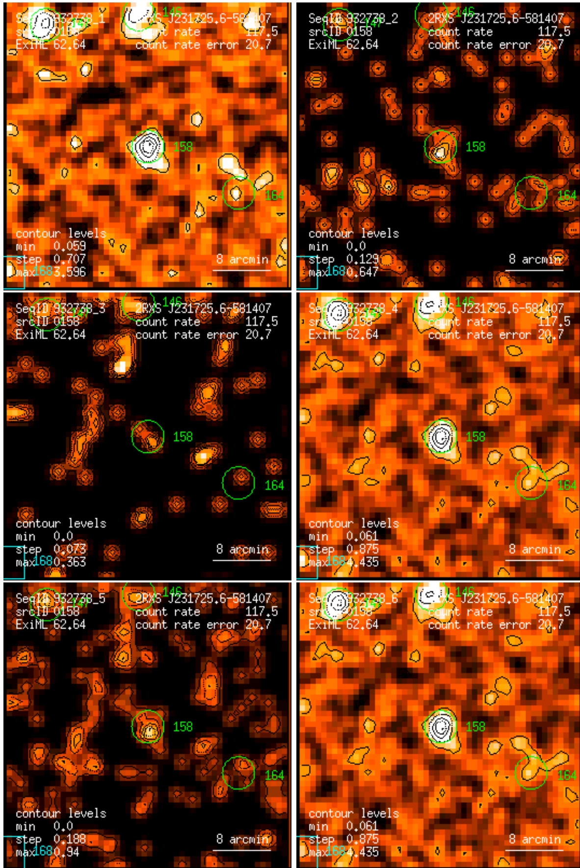
Figure 158: RASS 932738: detection 0158: band rate images, Gaussian filter: (1) PSPC channels 11 – 41, (2) 52 – 90, (3) 91 – 201, (4) 11 – 235, (5) 52 – 201, (6) 11 – 201. Broad band rates in counts/ks. Band rate contour levels in counts/ks/arcmin 2 .
