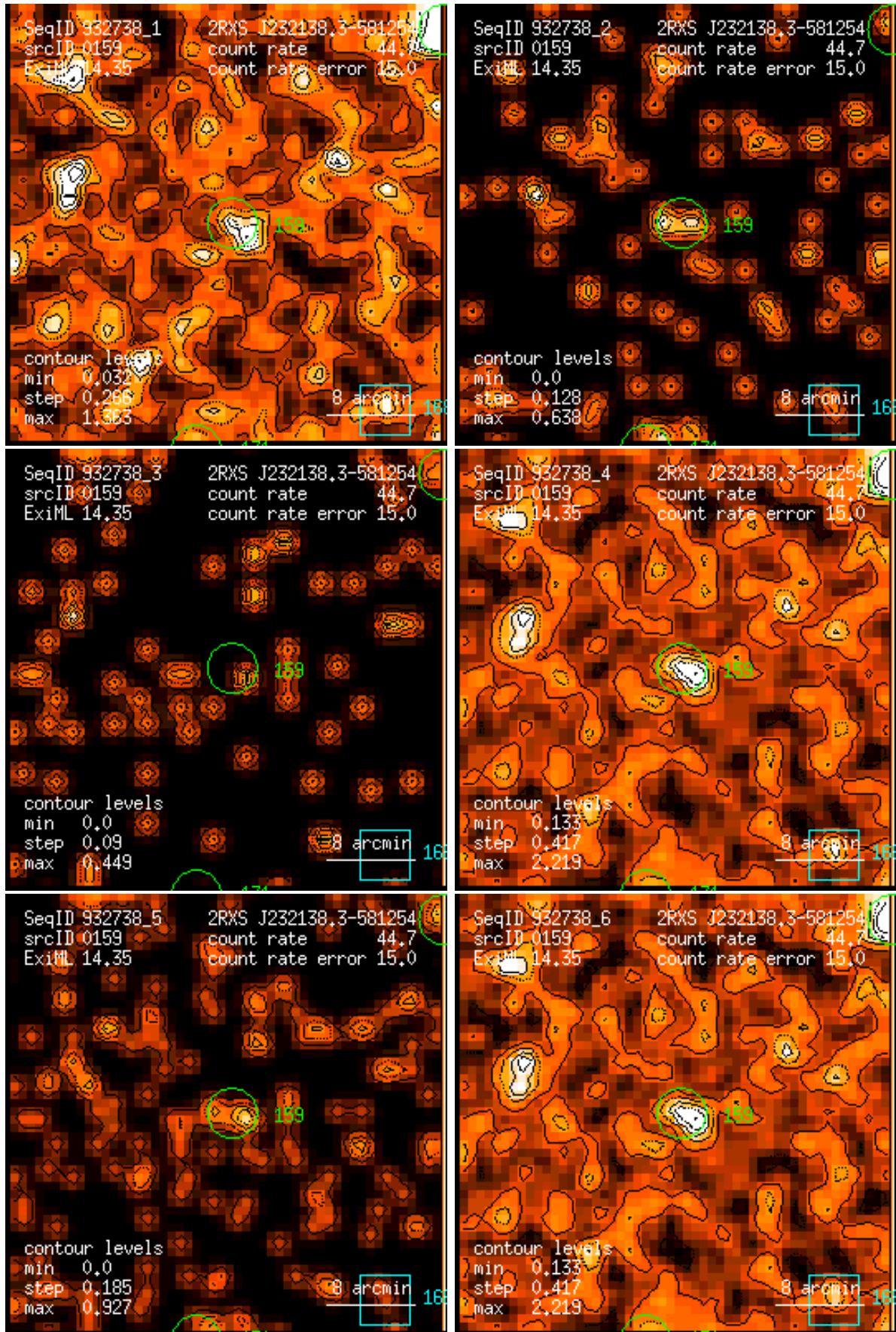
Figure 159: RASS 932738: detection 0159: band rate images, Gaussian filter: (1) PSPC channels 11 – 41, (2) 52 – 90, (3) 91 – 201, (4) 11 – 235, (5) 52 – 201, (6) 11 – 201. Broad band rates in counts/ks. Band rate contour levels in counts/ks/arcmin 2 .
