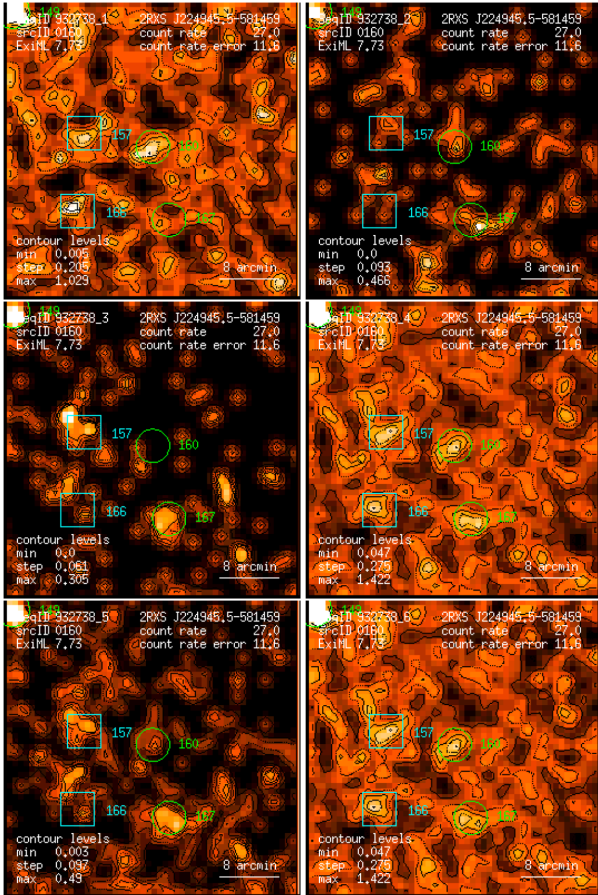
Figure 160: RASS 932738: detection 0160: band rate images, Gaussian filter: (1) PSPC channels 11 – 41, (2) 52 – 90, (3) 91 – 201, (4) 11 – 235, (5) 52 – 201, (6) 11 – 201. Broad band rates in counts/ks. Band rate contour levels in counts/ks/arcmin 2 .
