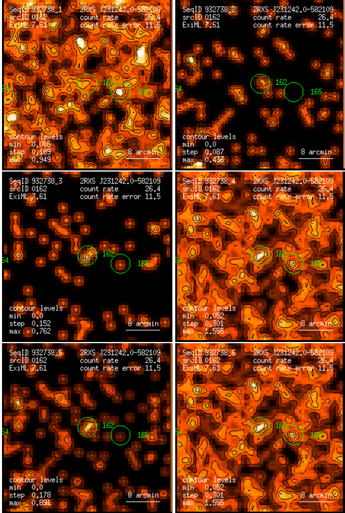
Figure 162: RASS 932738: detection 0162: band rate images, Gaussian filter: (1) PSPC channels 11 – 41, (2) 52 – 90, (3) 91 – 201, (4) 11 – 235, (5) 52 – 201, (6) 11 – 201. Broad band rates in counts/ks. Band rate contour levels in counts/ks/arcmin 2 .
