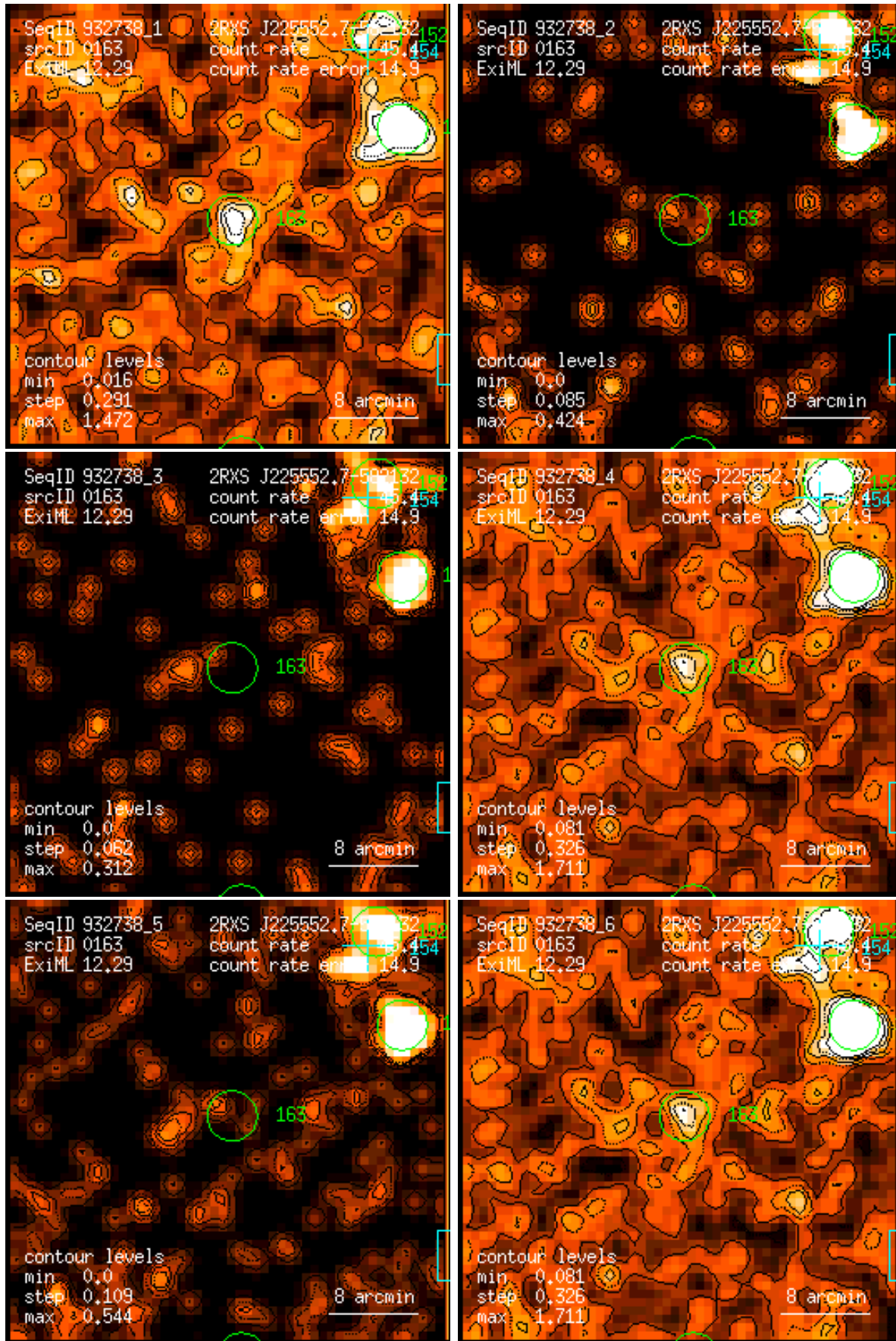
Figure 163: RASS 932738: detection 0163: band rate images, Gaussian filter: (1) PSPC channels 11 – 41, (2) 52 – 90, (3) 91 – 201, (4) 11 – 235, (5) 52 – 201, (6) 11 – 201. Broad band rates in counts/ks. Band rate contour levels in counts/ks/arcmin 2 .
