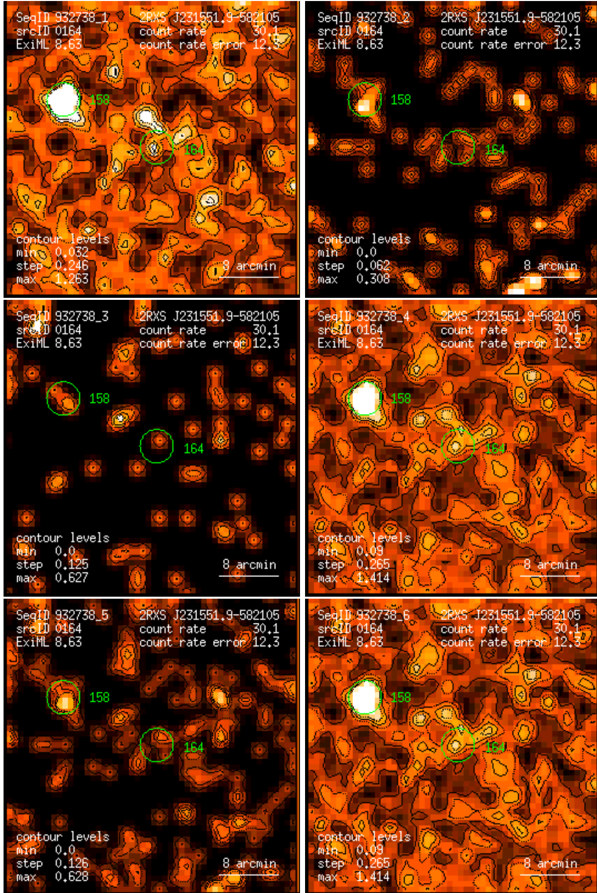
Figure 164: RASS 932738: detection 0164: band rate images, Gaussian filter: (1) PSPC channels 11 – 41, (2) 52 – 90, (3) 91 – 201, (4) 11 – 235, (5) 52 – 201, (6) 11 – 201. Broad band rates in counts/ks. Band rate contour levels in counts/ks/arcmin 2 .
