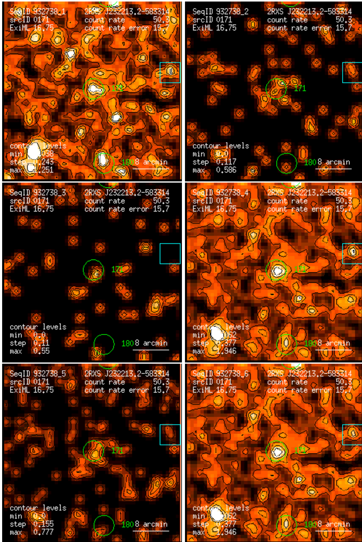
Figure 171: RASS 932738: detection 0171: band rate images, Gaussian filter: (1) PSPC channels 11 – 41, (2) 52 – 90, (3) 91 – 201, (4) 11 – 235, (5) 52 – 201, (6) 11 – 201. Broad band rates in counts/ks. Band rate contour levels in counts/ks/arcmin 2 .
