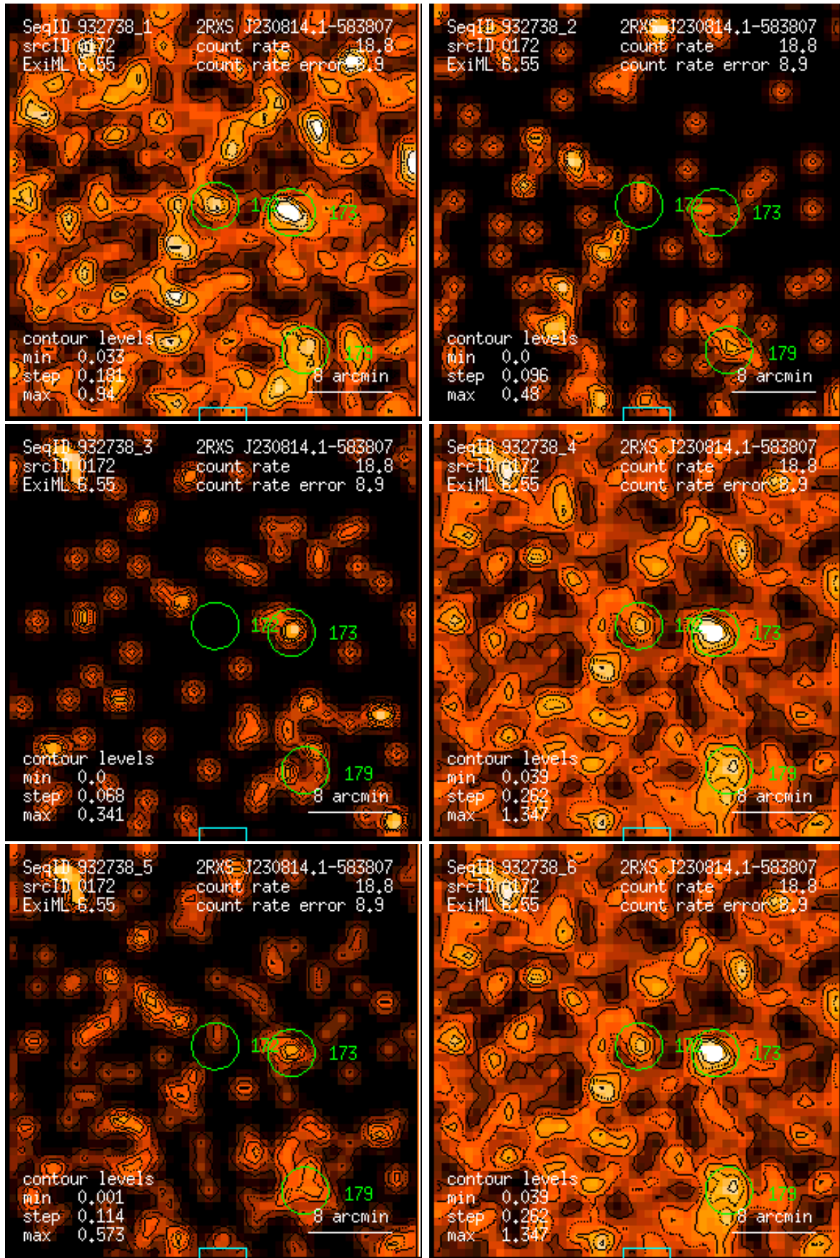
Figure 172: RASS 932738: detection 0172: band rate images, Gaussian filter: (1) PSPC channels 11 – 41, (2) 52 – 90, (3) 91 – 201, (4) 11 – 235, (5) 52 – 201, (6) 11 – 201. Broad band rates in counts/ks. Band rate contour levels in counts/ks/arcmin 2 .
