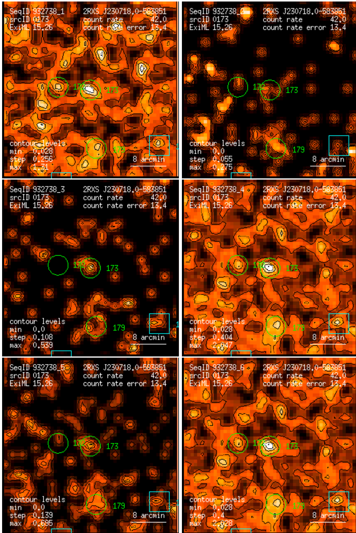
Figure 173: RASS 932738: detection 0173: band rate images, Gaussian filter: (1) PSPC channels 11 – 41, (2) 52 – 90, (3) 91 – 201, (4) 11 – 235, (5) 52 – 201, (6) 11 – 201. Broad band rates in counts/ks. Band rate contour levels in counts/ks/arcmin 2 .
