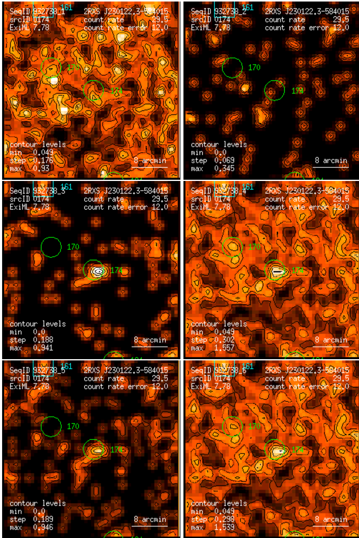
Figure 174: RASS 932738: detection 0174: band rate images, Gaussian filter: (1) PSPC channels 11 – 41, (2) 52 – 90, (3) 91 – 201, (4) 11 – 235, (5) 52 – 201, (6) 11 – 201. Broad band rates in counts/ks. Band rate contour levels in counts/ks/arcmin 2 .
